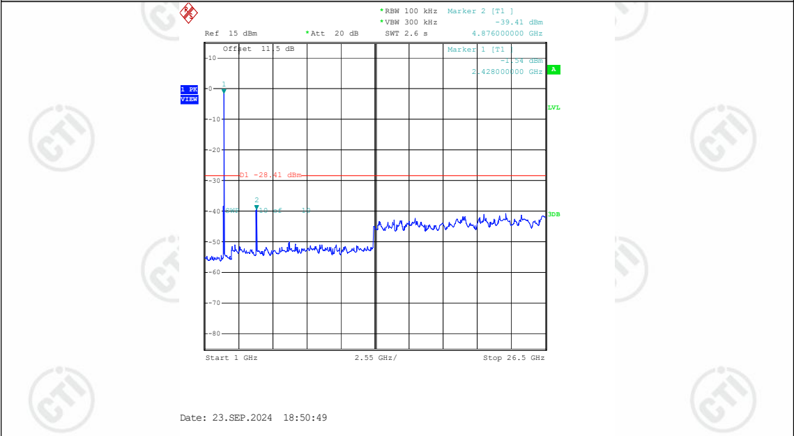
11N20SISO-Ant1-2437-1000~26500-PASS
