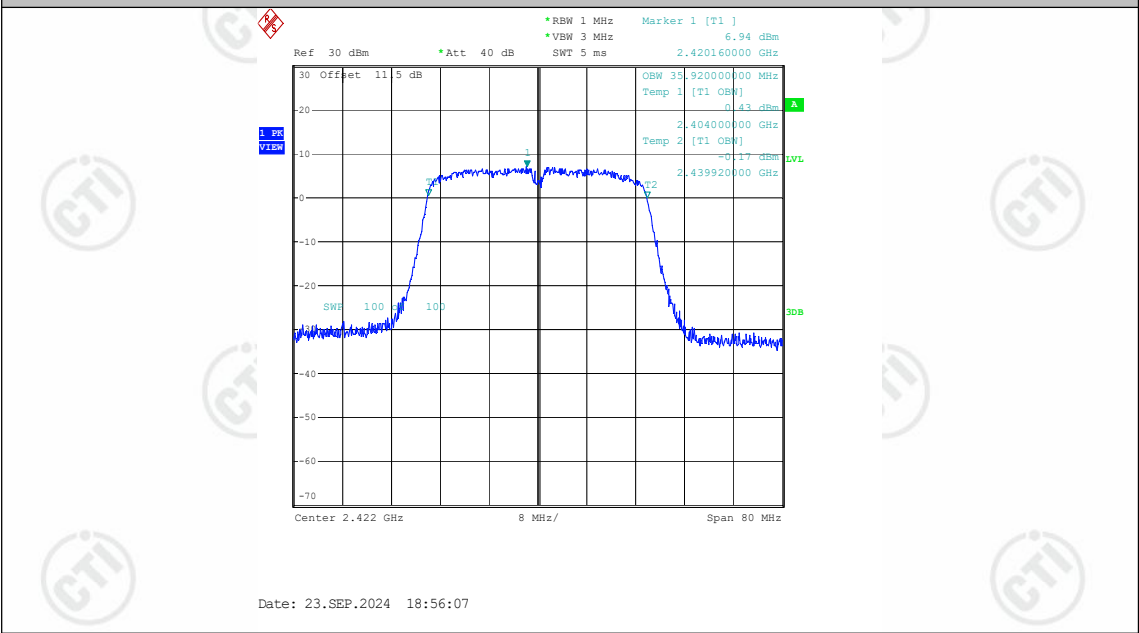
11N40SISO-Ant1-2422
