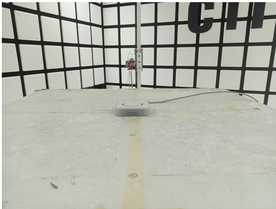
Radiated spurious emission Test Setup-2(Above 1GHz)(new)
