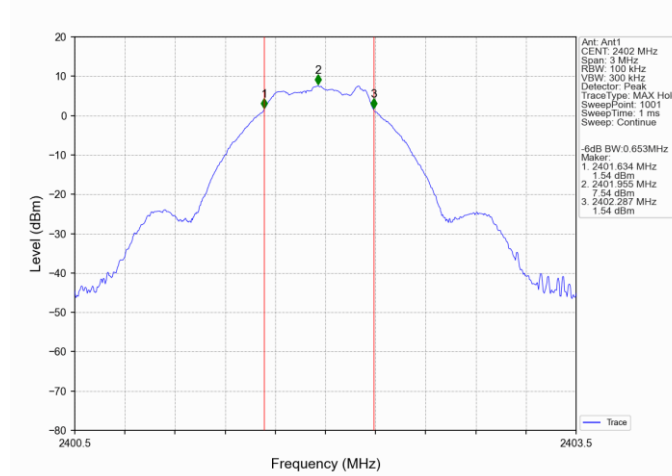
1M_LCH_2402MHz_Ant1_NTNV
