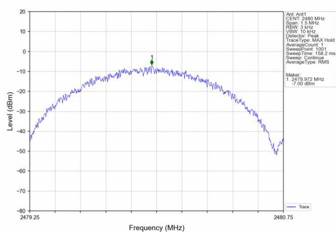
1M_HCH_2480MHz_Ant1_NTNV
