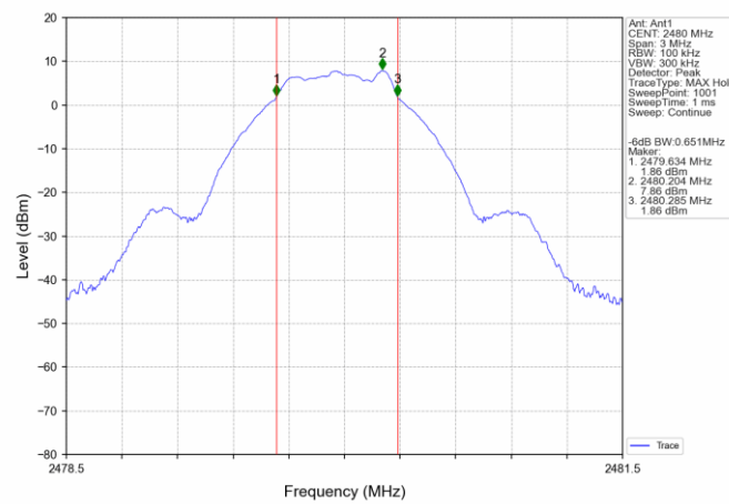
1M_HCH_2480MHz_Ant1_NTNV
