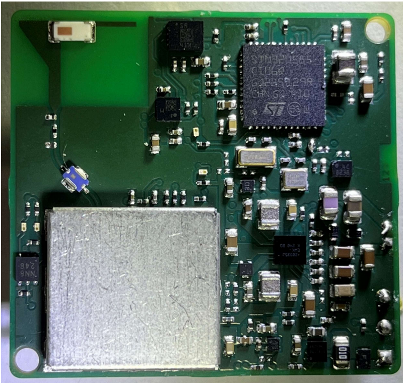
Figure 1 - Module Front
