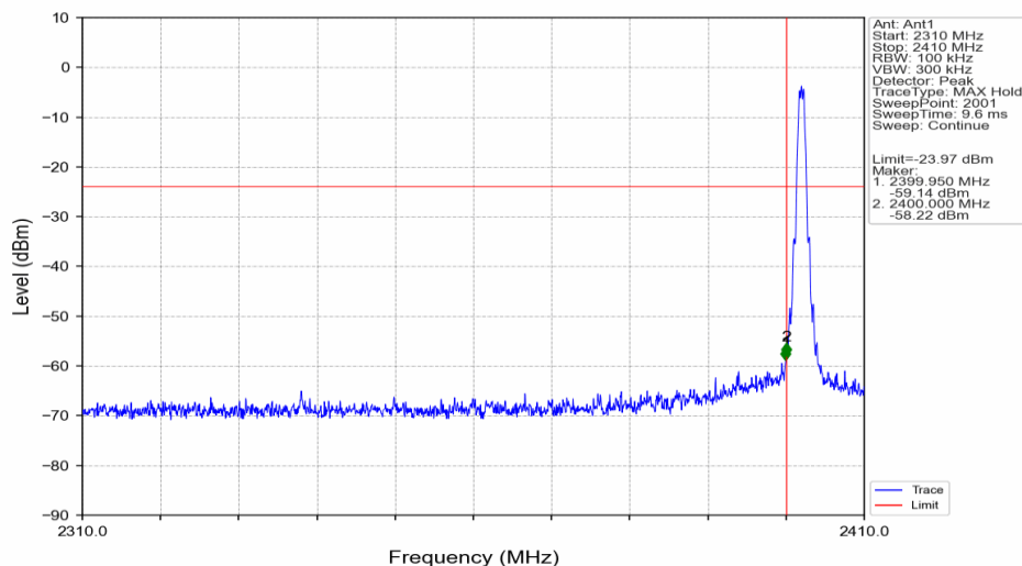
1M_LCH_2402MHz_Ant1_NTNV
