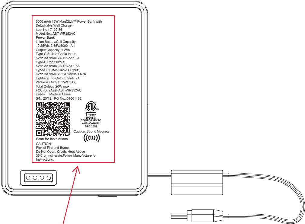
Wireless Power Bank Part
