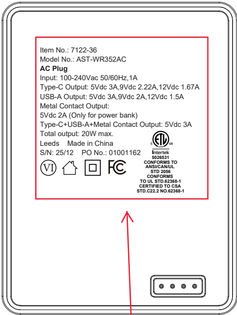
AC Plug Part
