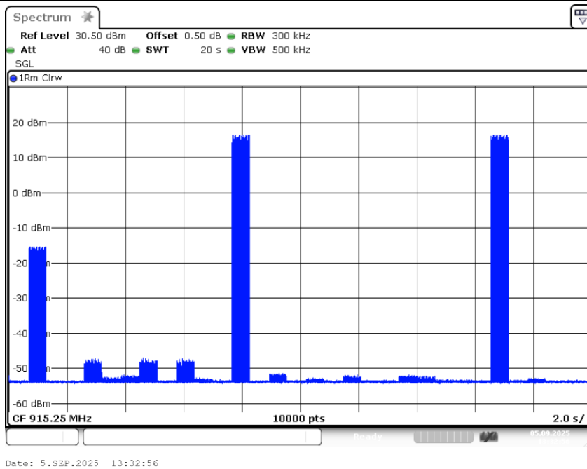
RF ID_Ant J4_915.25 - 2
