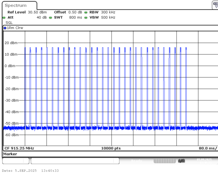
RF ID_Ant J4_915.25 - 1
