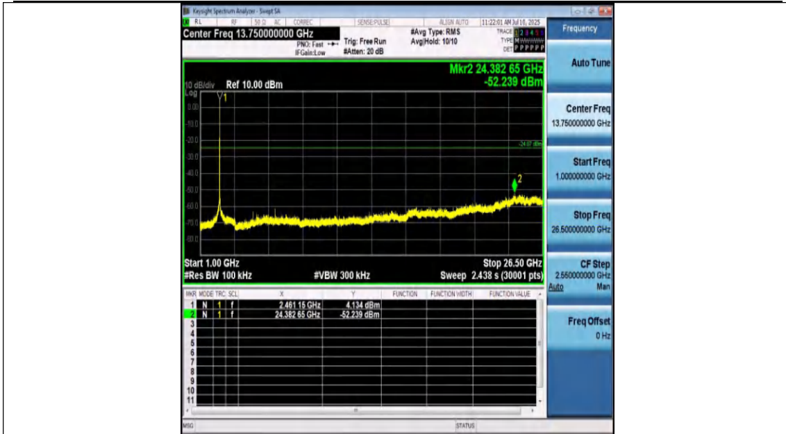
11B-Ant1-2462-1000~26500-PASS
