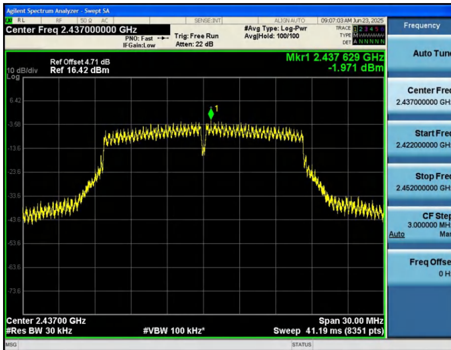
Power_Spectral_Density_HVNT_ANT1_802_11g_2437
