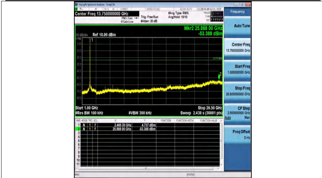
11N20SISO-Ant1-2462-1000~26500-PASS
