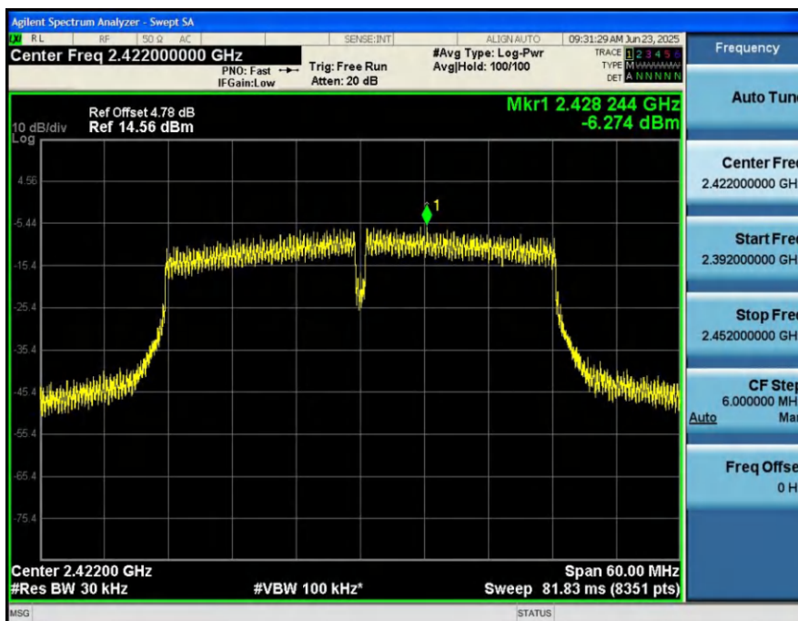
Power_Spectral_Density_HVNT_ANT1_802_11n(HT40)_2422
