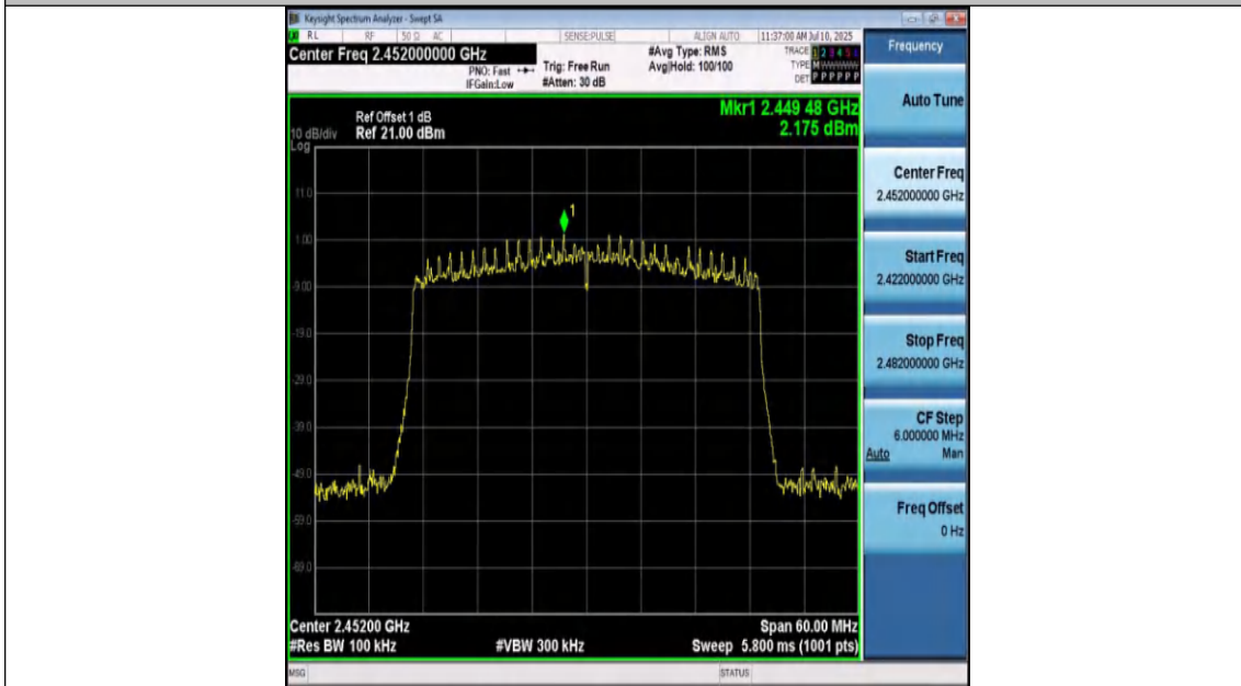
11AX40SISO-Ant1-2452-0~Reference-PASS
