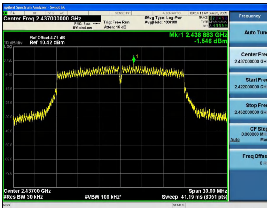
Power_Spectral_Density_HVNT_ANT1_802_11n(HT20)_2437
