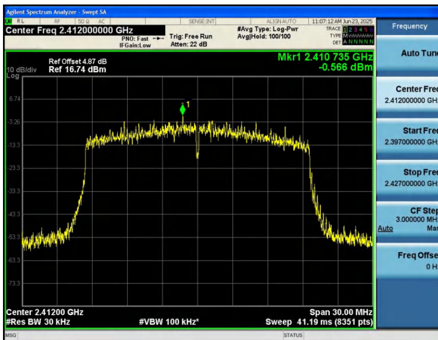
Power_Spectral_Density_HVNT_ANT1_802_11ax(HE20)_2412
