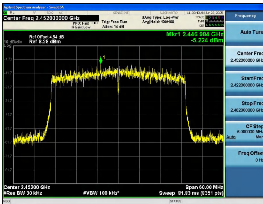
Power_Spectral_Density_HVNT_ANT1_802_11ax(HE40)_2452
