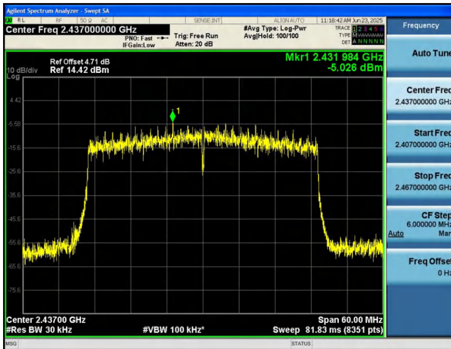
Power_Spectral_Density_HVNT_ANT1_802_11ax(HE40)_2437
