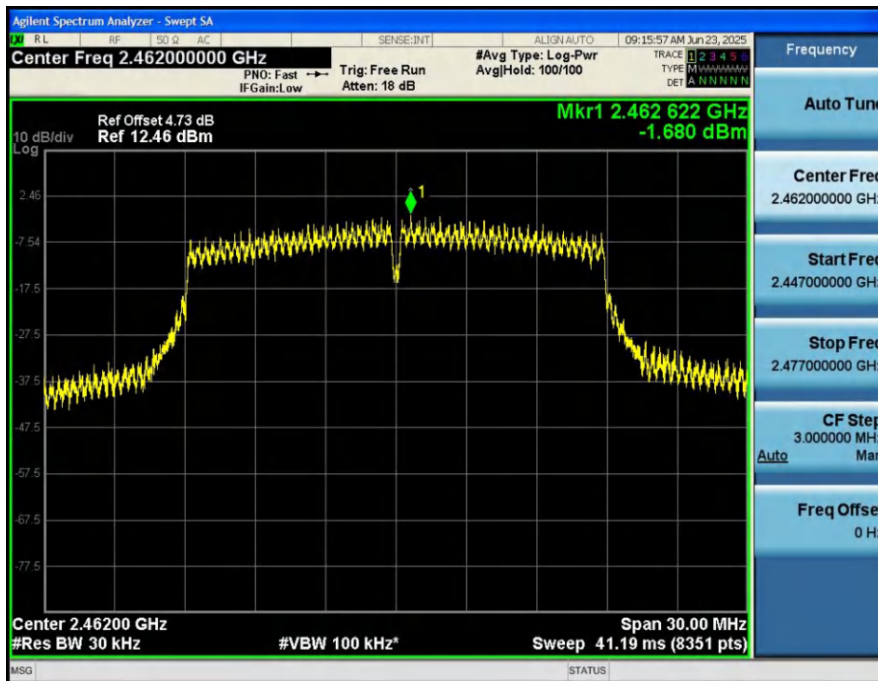
Power_Spectral_Density_HVNT_ANT1_802_11n(HT20)_2462
