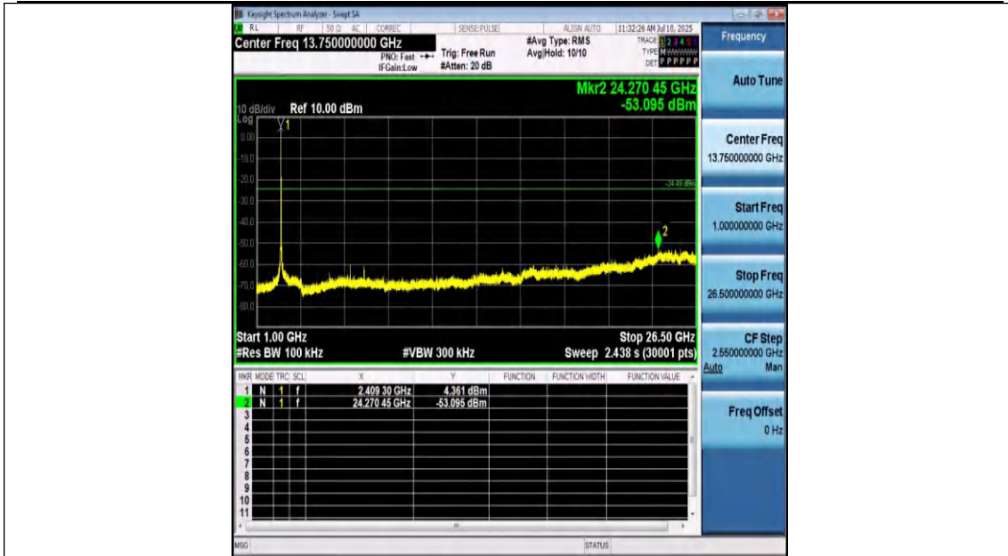
11AX20SISO-Ant1-2412-1000~26500-PASS
