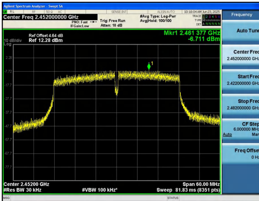
Power_Spectral_Density_HVNT_ANT1_802_11n(HT40)_2452
