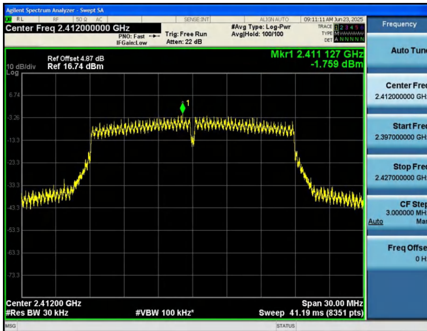
Power_Spectral_Density_HVNT_ANT1_802_11n(HT20)_2412
