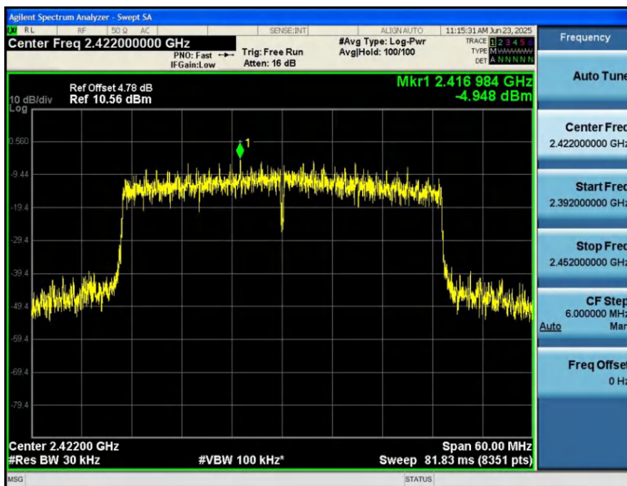
Power_Spectral_Density_HVNT_ANT1_802_11ax(HE40)_2422
