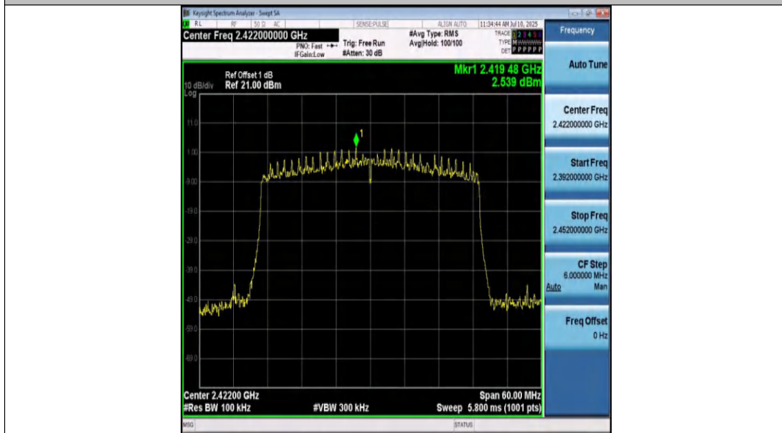
11AX40SISO-Ant1-2422-0~Reference-PASS
