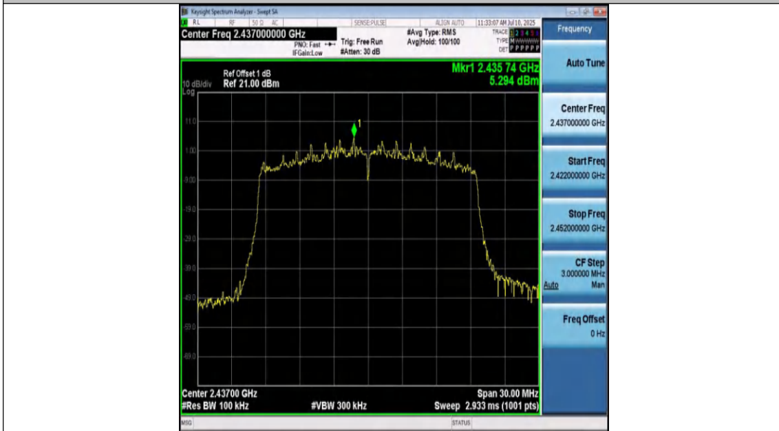
11AX20SISO-Ant1-2437-0~Reference-PASS
