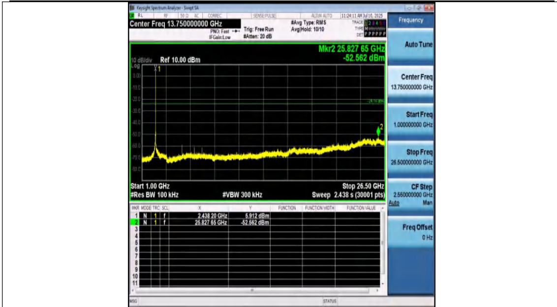
11G-Ant1-2437-1000~26500-PASS
