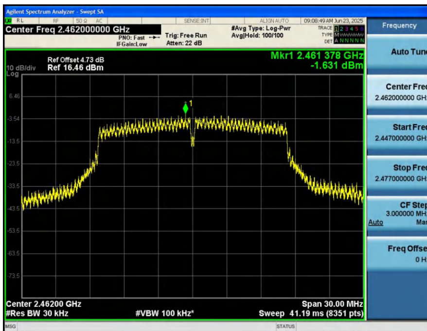
Power_Spectral_Density_HVNT_ANT1_802_11g_2462
