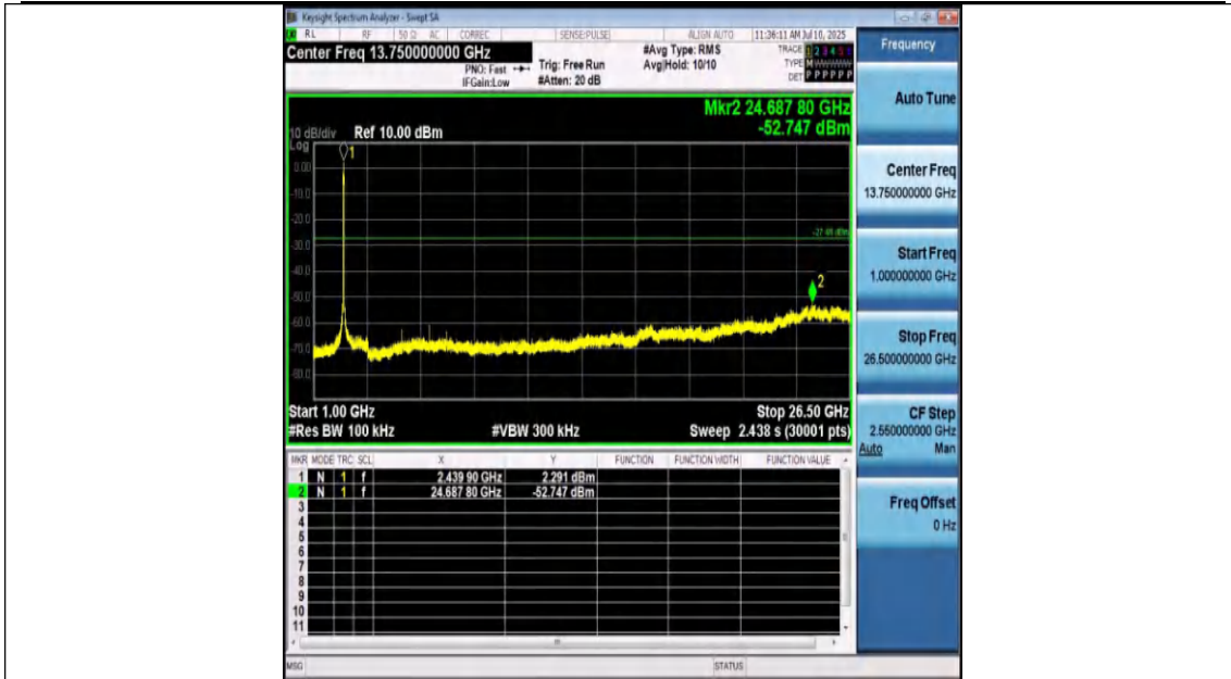
11AX40SISO-Ant1-2437-1000~26500-PASS
