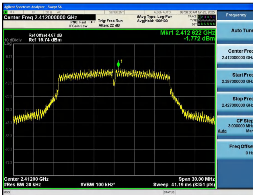
Power_Spectral_Density_HVNT_ANT1_802_11g_2412
