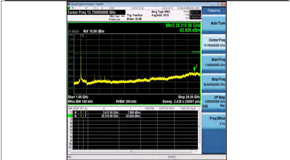
11N20SISO-Ant1-2412-1000~26500-PASS
