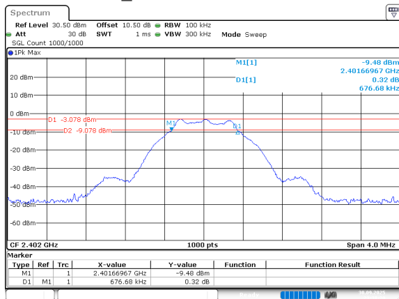
2.4G_SRD_1M_Low_Channel
