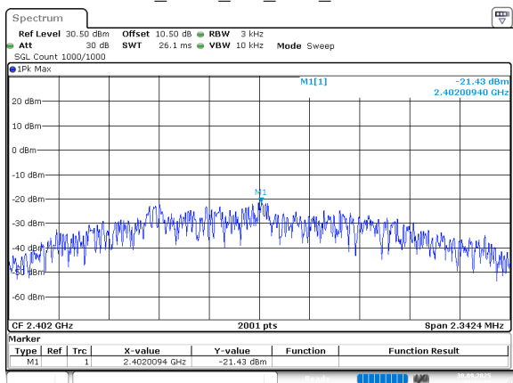
2.4G_SRD_2M_Low_Channel
