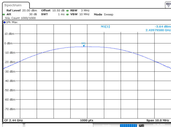
2.4G_SRD_2M_Middle_Channel
