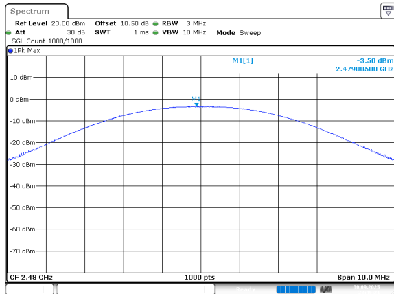
2.4G_SRD_1M_High_Channel
