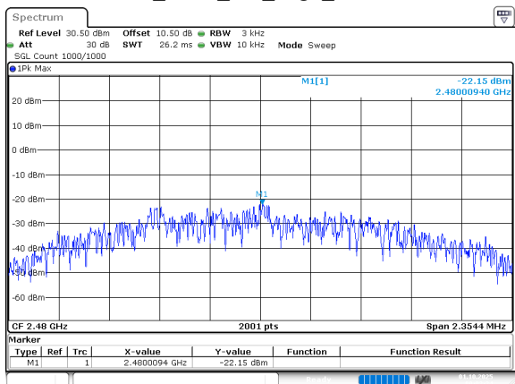
2.4G_SRD_2M_High_Channel
