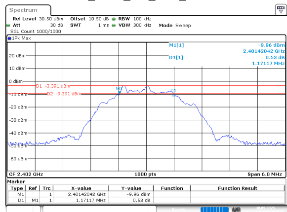
2.4G_SRD_2M_Low_Channel
