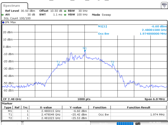
2.4G_SRD_2M_High_Channel
