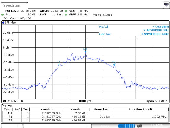
2.4G_SRD_2M_Low_Channel
