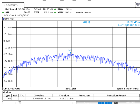
2.4G_SRD_1M_Low_Channel
