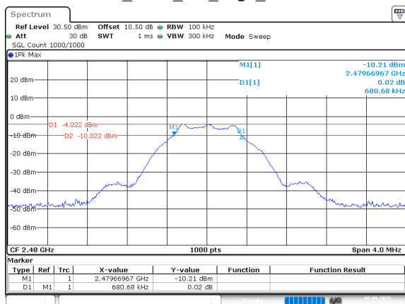
2.4G_SRD_1M_High_Channel
