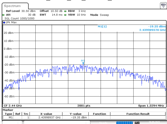
2.4G_SRD_1M_Middle_Channel
