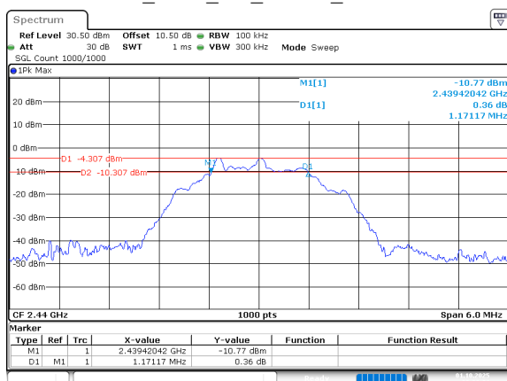
2.4G_SRD_2M_Middle_Channel
