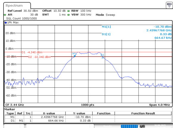
2.4G_SRD_1M_Middle_Channel
