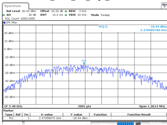
2.4G_SRD_1M_High_Channel
