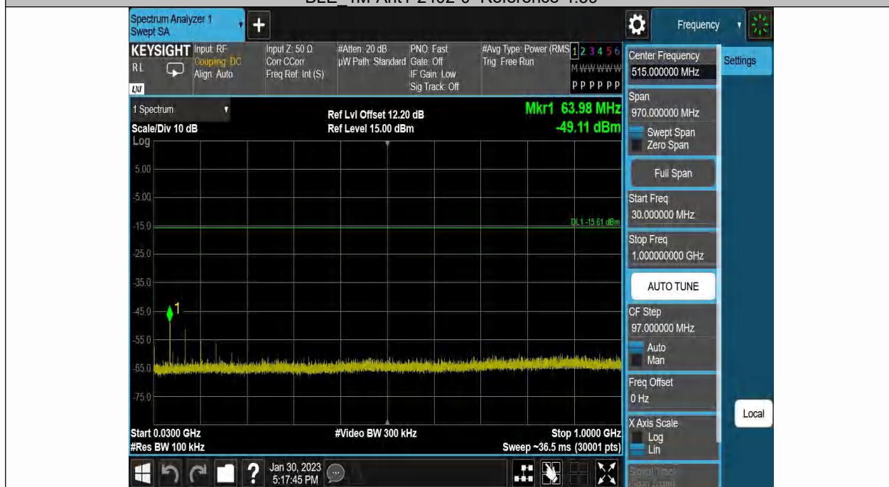
BLE_1M-Ant1-2402-30~1000-4.39
