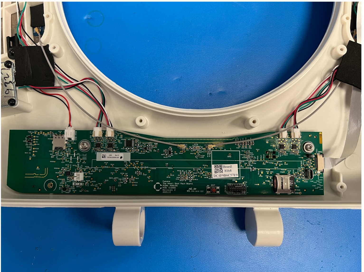
Close Up of the PCB Installed in the Top Half
