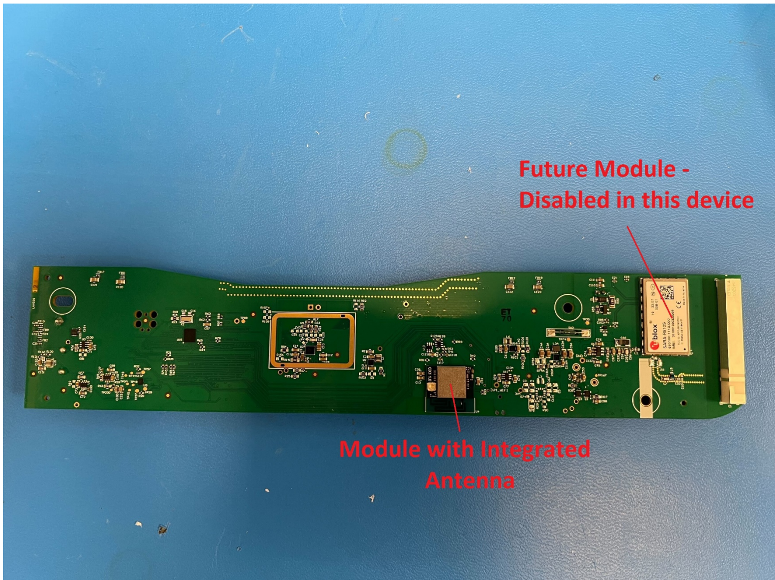
PCB Board RF Side
