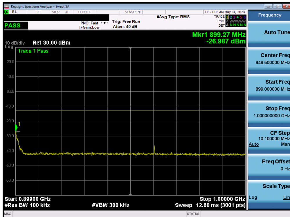
Plot 7-20. Conducted Spurious Plot (LTE Band 26/5 – High Channel)
