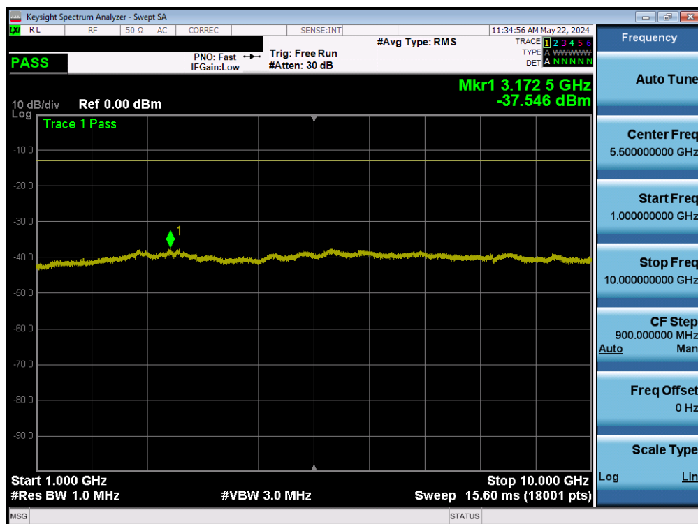
Plot 7-18. Conducted Spurious Plot (LTE Band 26/5 – Mid Channel)
