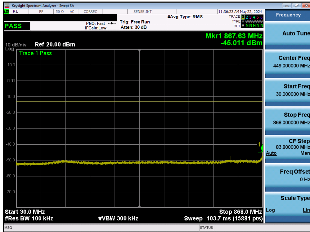
Plot 7-19. Conducted Spurious Plot (LTE Band 26/5 – High Channel)
