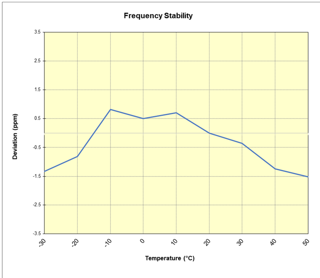
Plot 7-61. WCDMA 850 Frequency Stability Chart
