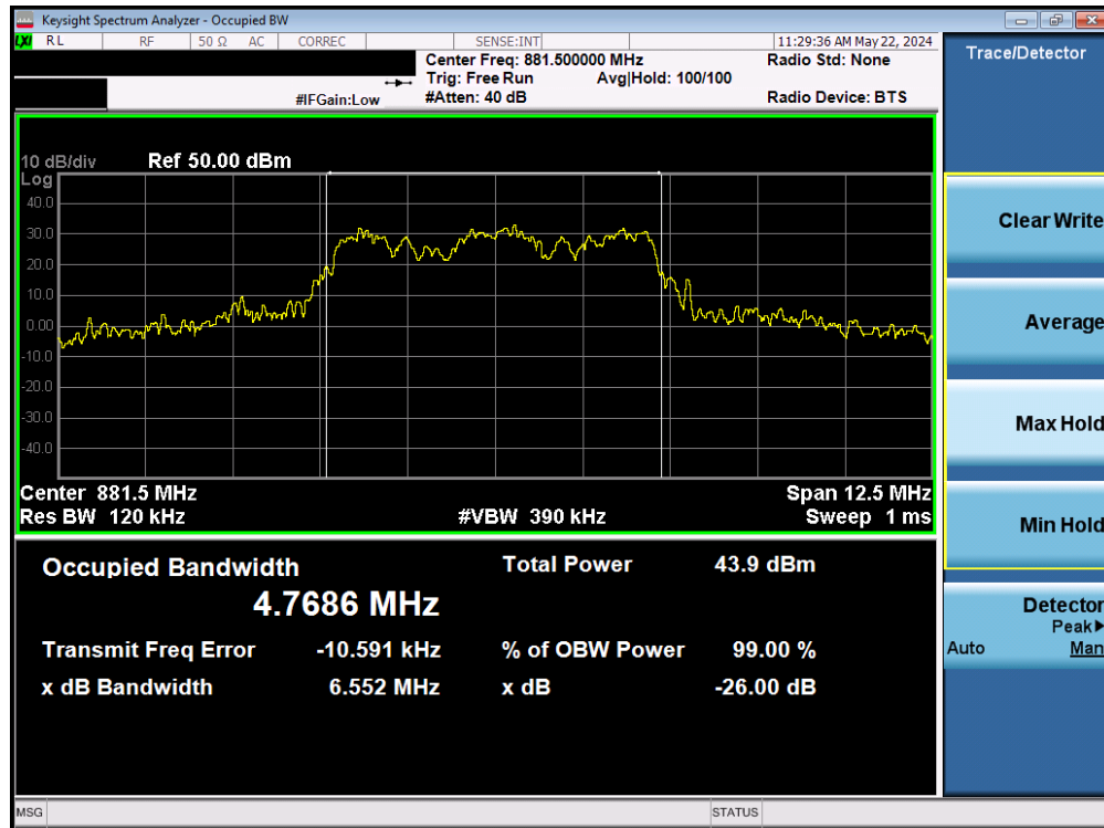
Plot 7-10. Occupied Bandwidth Plot (LTE Band 26/5)
