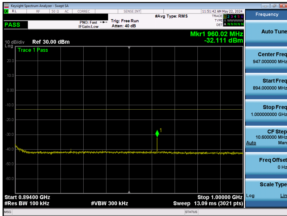
Plot 7-26. Conducted Spurious Plot (WCDMA Cell – Mid Channel)
