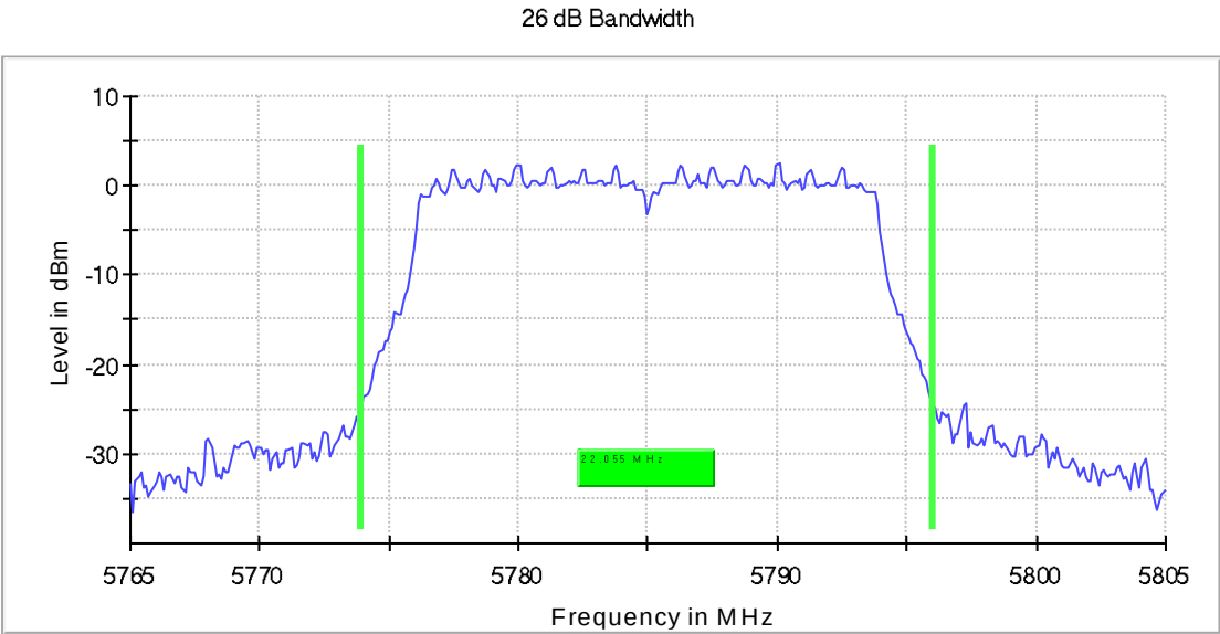
Fig. 96: Middle Channel - Emission Bandwidth 26 dB
