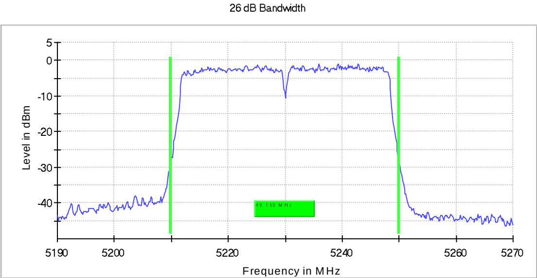
Fig. 28: High Channel - Emission Bandwidth 26 dB
