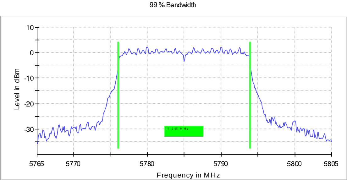
Fig. 95: Middle Channel - 99% Occupied Channel Bandwidth
