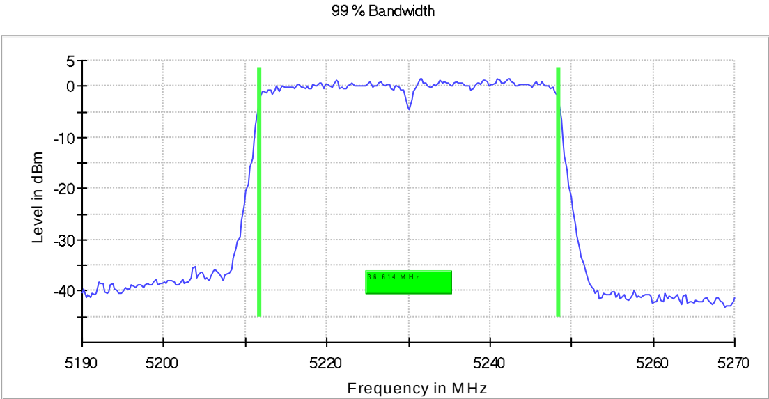
Fig. 27: High Channel - 99% Occupied Channel Bandwidth
