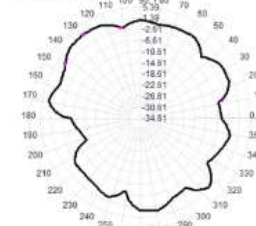
Total(H+V), Max= 1.76dBi, Crd=15.80
