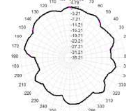
Total(H+V), Max= 1.58dBi, Crd=13.41
