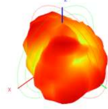
2450.0MHz H+V, Eff: 61.3%
