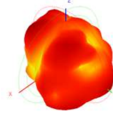
2400.0MHz H+V, Eff: 63.8%
