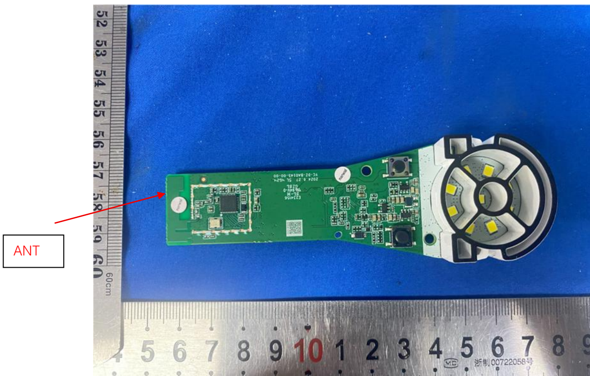
Internal Photo
