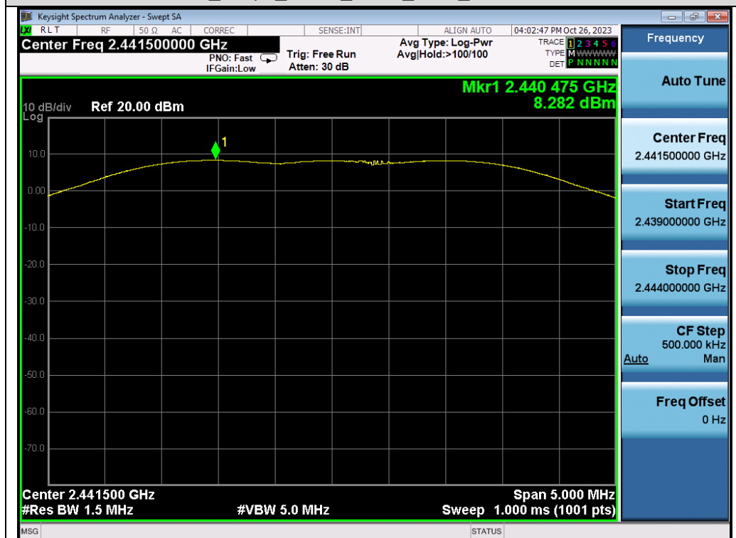
Test_Graph_GFSK_ANT1_2441.5_Peak Power
