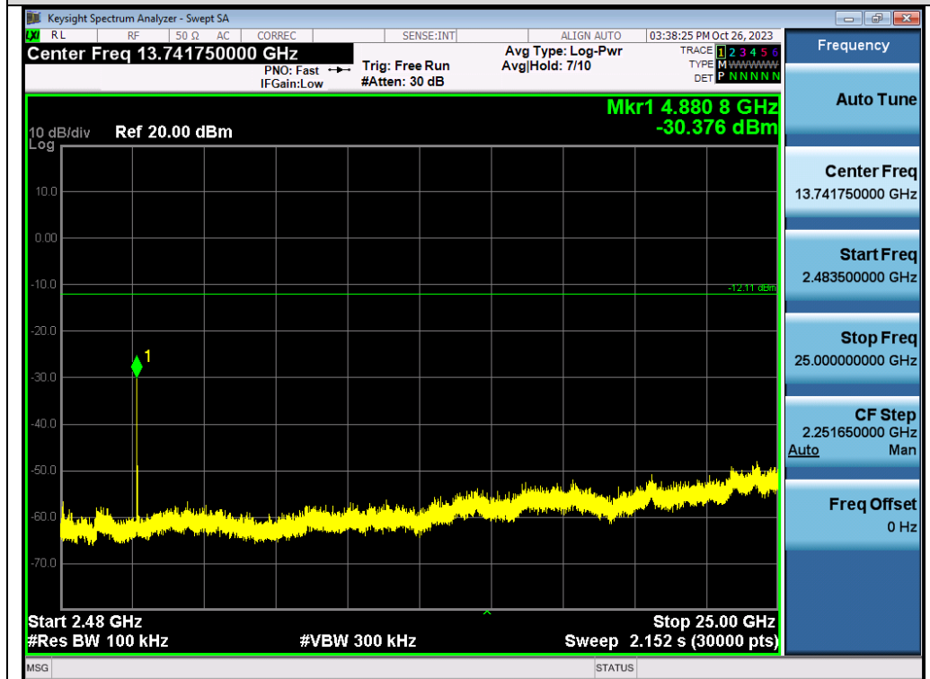
Test_Graph_GFSK_ANT1_2441.5_Higher Band Emissions
