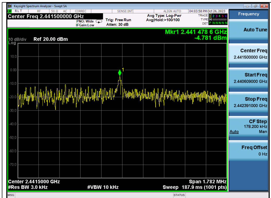
Test_Graph_GFSK_ANT1_2441.5_PSD
