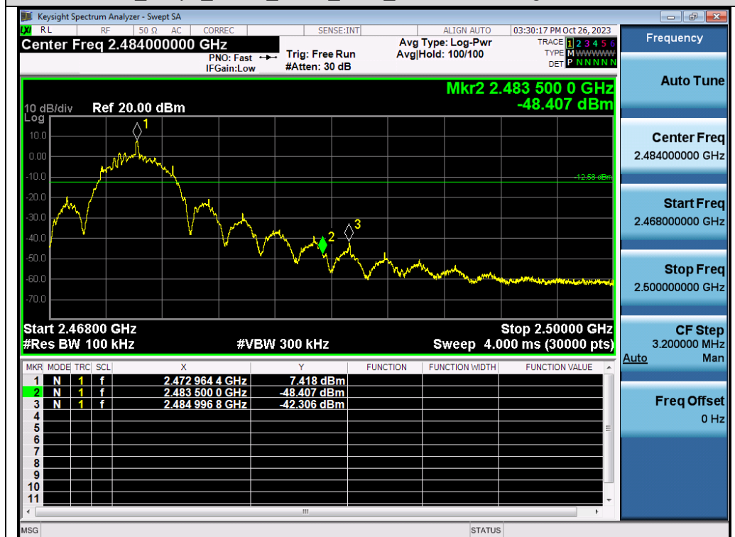
Test_Graph_GFSK_ANT1_2473_Higher Band Edge Emissions
