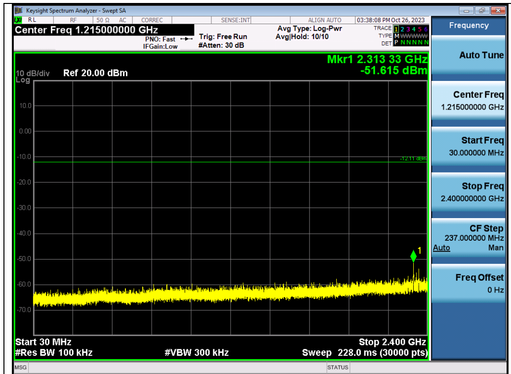
Test_Graph_GFSK_ANT1_2441.5_Lower Band Emissions
