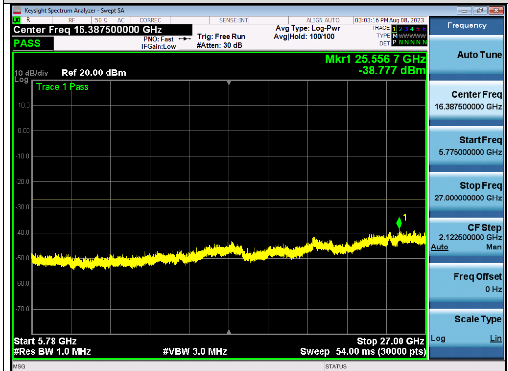
Test_Graph_802.11ac80_ANT2_5610_MCS9_Frequency Band 4
