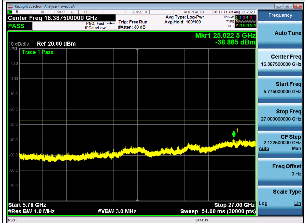
Test_Graph_802.11n40_ANT1_5590_MCS0_Frequency Band 4
