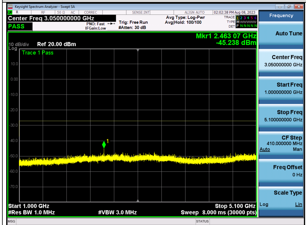
Test_Graph_802.11a_ANT2_5260_6Mbps_Frequency Band 2
