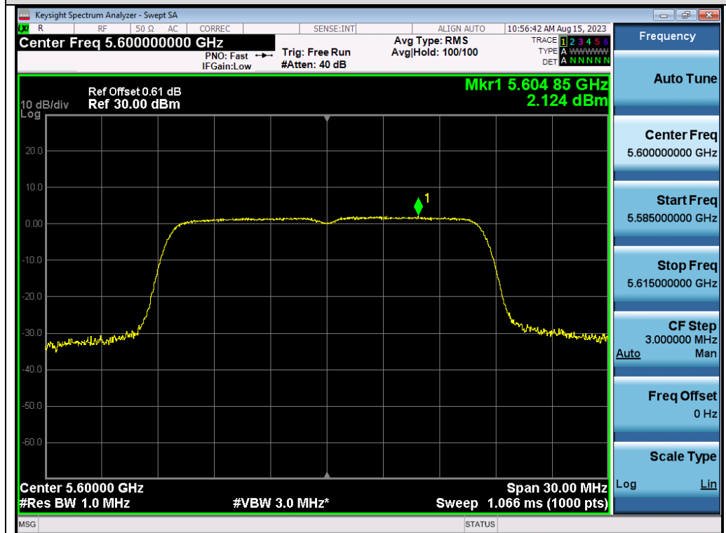
Test_Graph_802.11a_ANT2_5600_6Mbps_PSD
