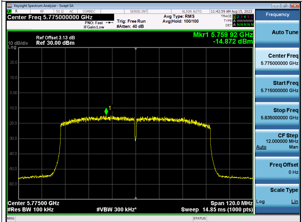
Test_Graph_802.11ac80_ANT2_5775_MCS9_PSD
