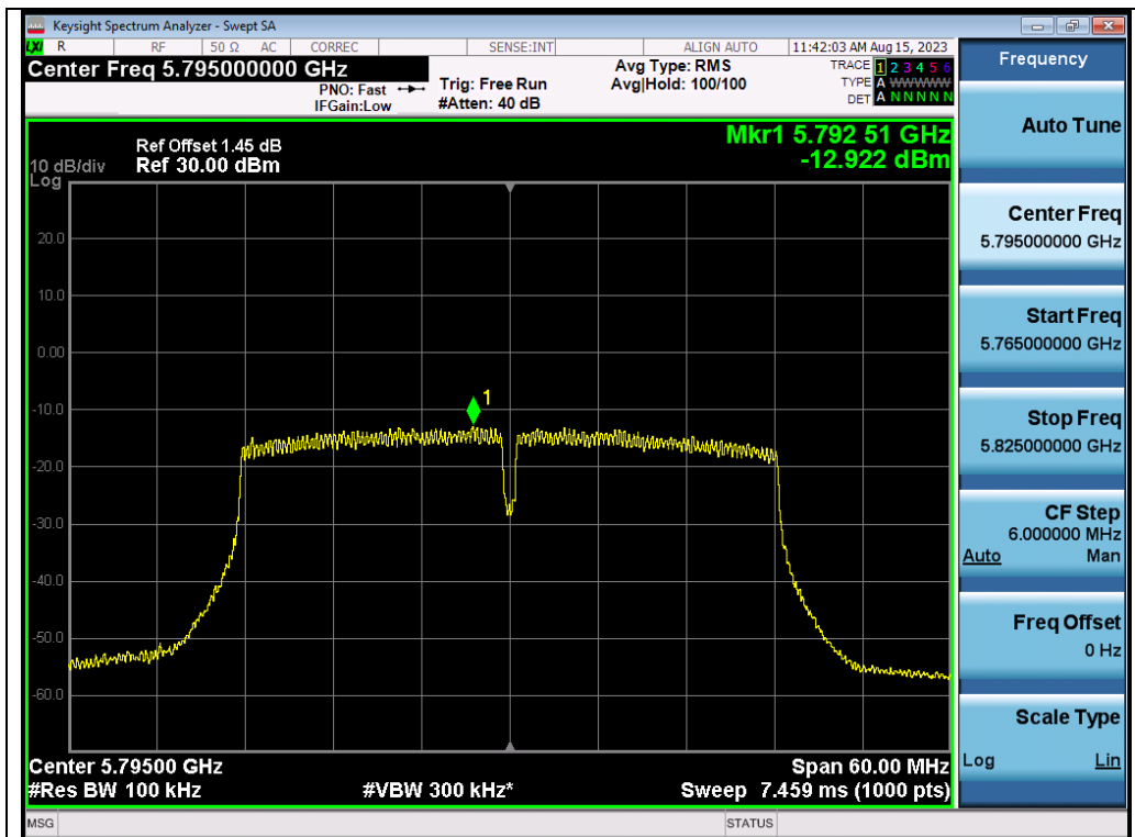
Test_Graph_802.11ac40_ANT2_5795_MCS9_PSD
