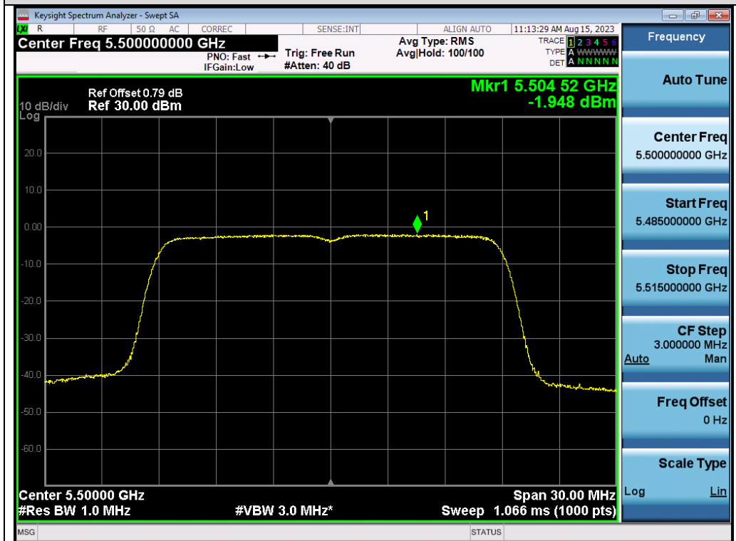
Test_Graph_802.11ac20_ANT2_5500_MCS0_PSD
