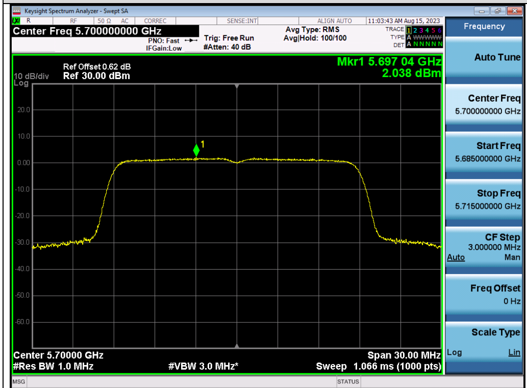
Test_Graph_802.11n20_ANT2_5700_MCS0_PSD
