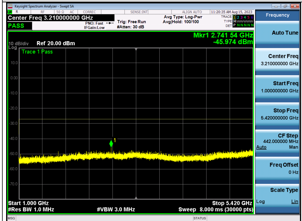
Test_Graph_802.11ac80_ANT2_5530_MCS9_Frequency Band 2
