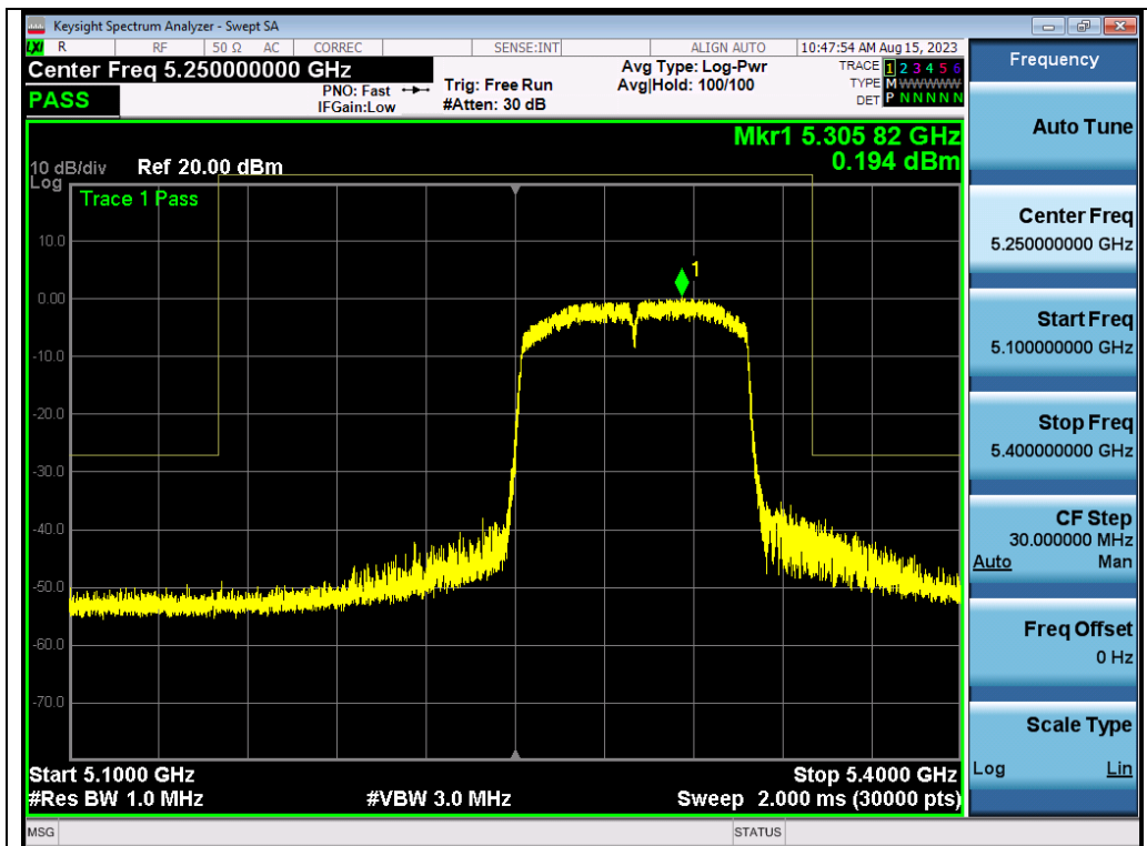
Test_Graph_802.11ac80_ANT2_5290_MCS9_Frequency Band 3
