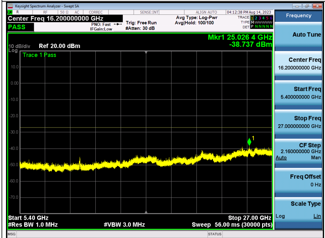
Test_Graph_802.11n40_ANT1_5270_MCS0_Frequency Band 4
