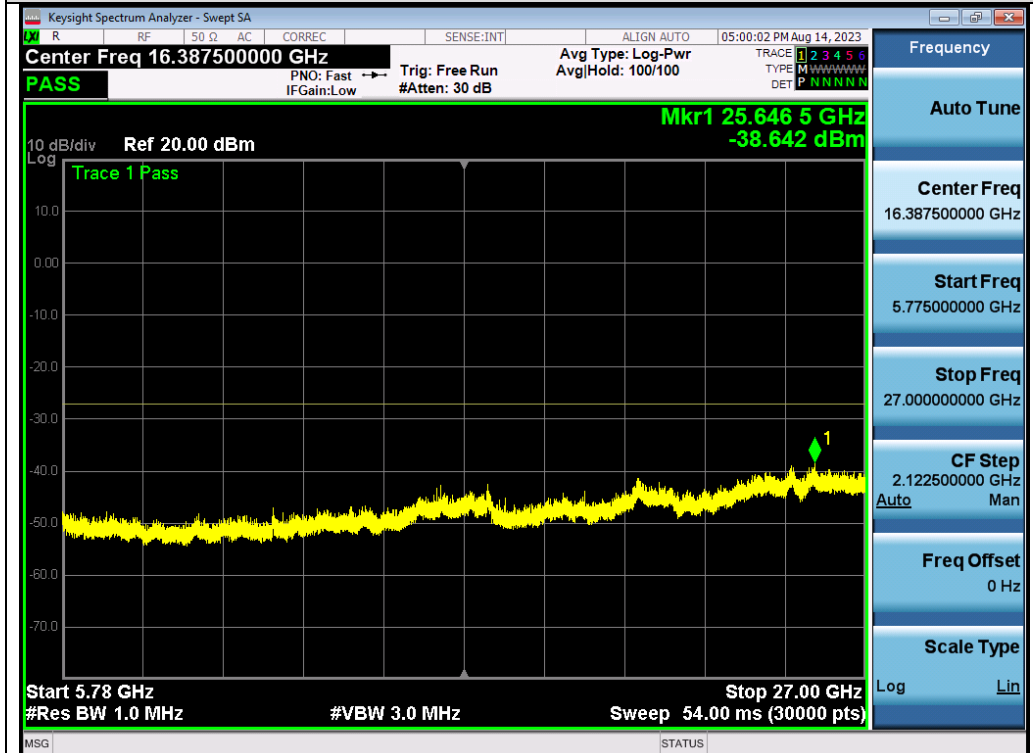
Test_Graph_802.11n40_ANT1_5670_MCS0_Frequency Band 4
