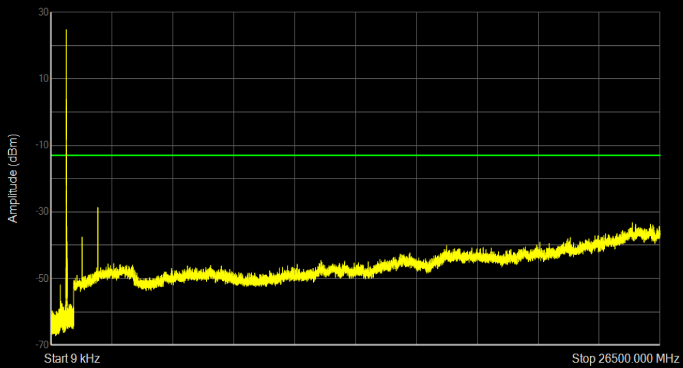
Band71 QPSK BW=15MHz Channel=133397 RB Size=1 Position=#0
