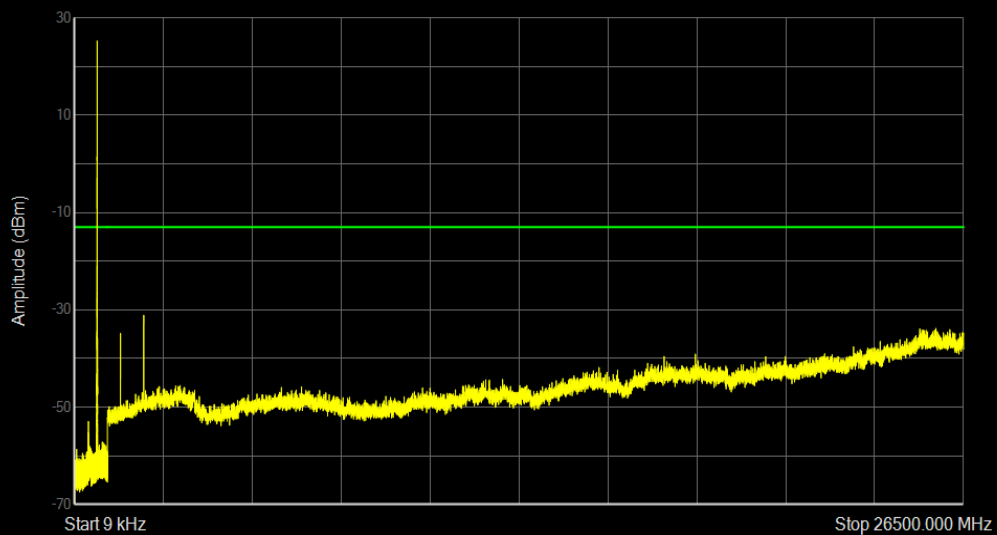
Band71 QPSK BW=5MHz Channel=133447 RB Size=1 Position=#0
