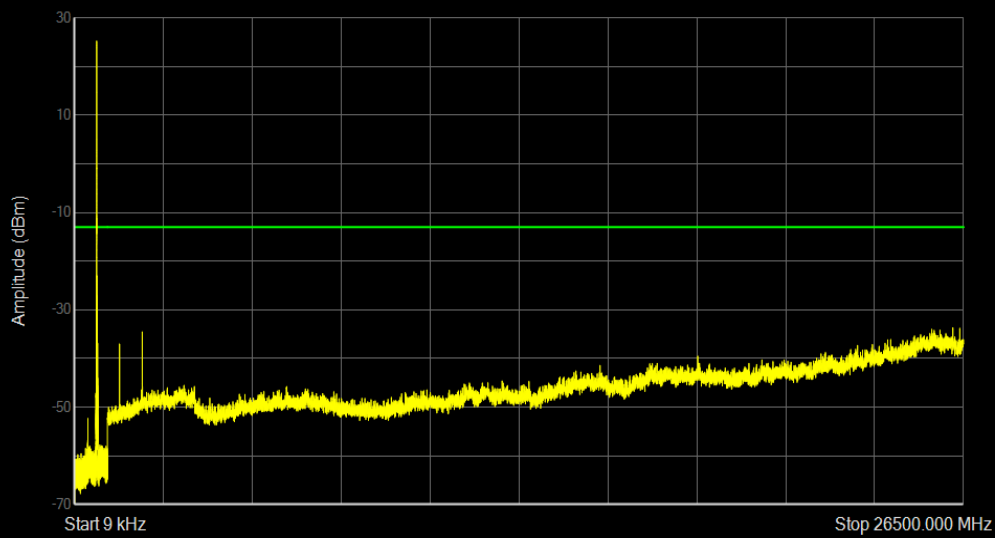
Band71 QPSK BW=20MHz Channel=133372 RB Size=1 Position=#0
