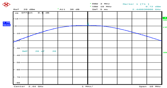
Middle 0.72dBm
