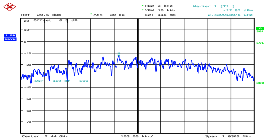
Middle -12.87dBm/3kHz
