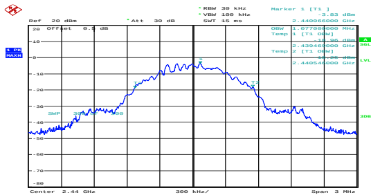
Middle 1.077MHz
