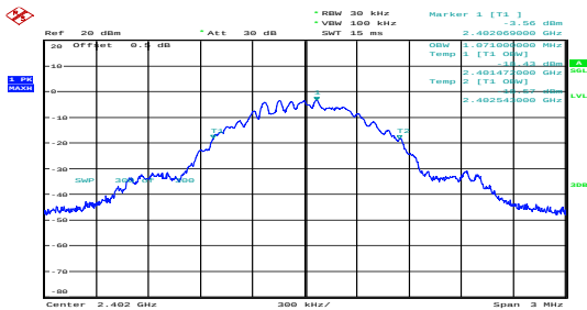
Low 1.071MHz
