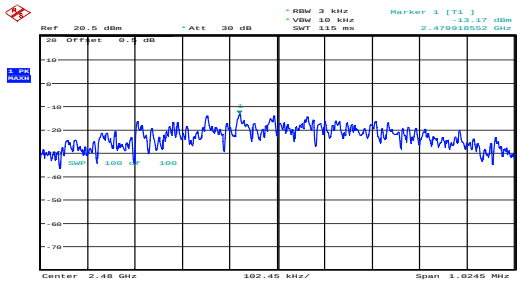
High -13.17dBm/3kHz
