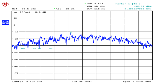
Low -12.59dBm/3kHz
