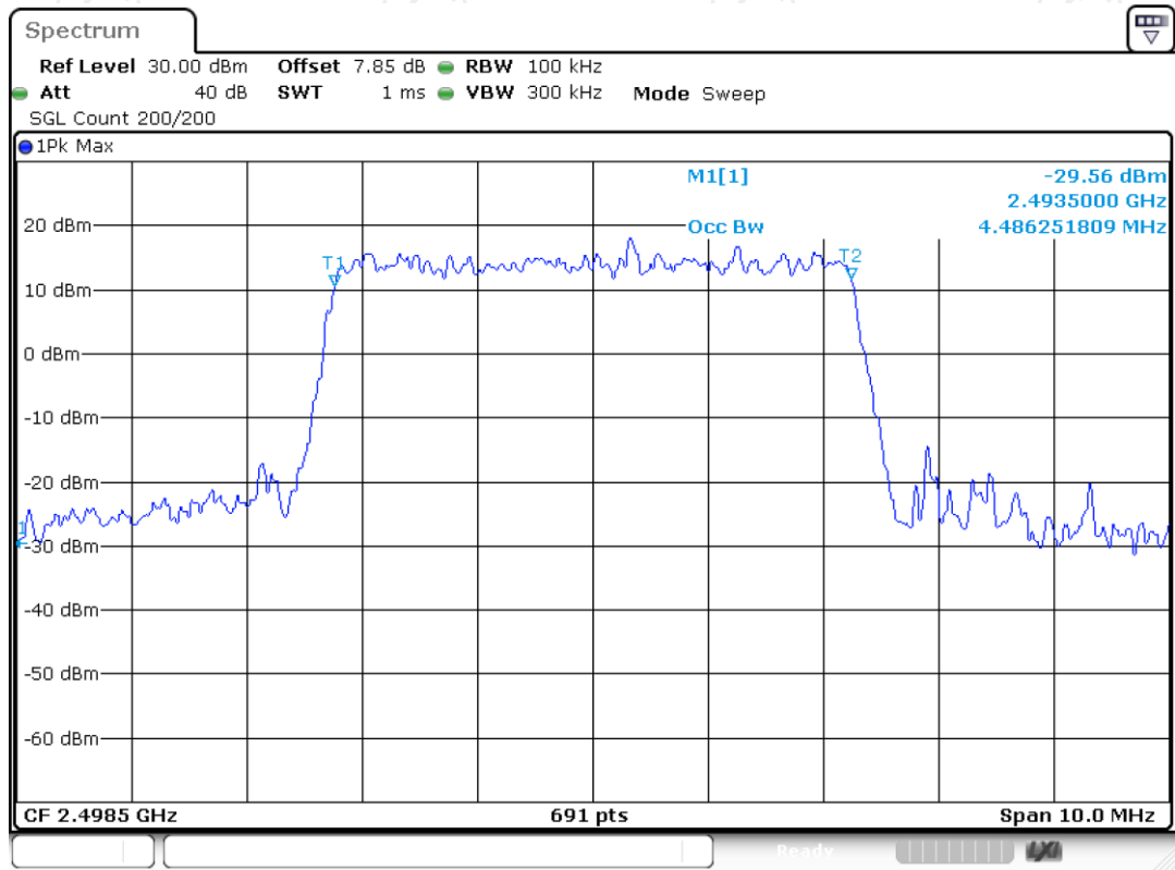
Band41 QPSK BW=5MHz Channel=39675 RB Size=25 Position=#0
