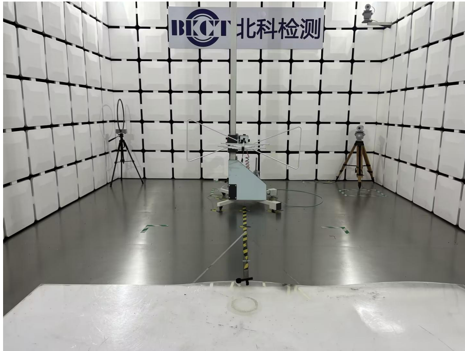
FCC ID:2A95L-SX25 Test Photo
