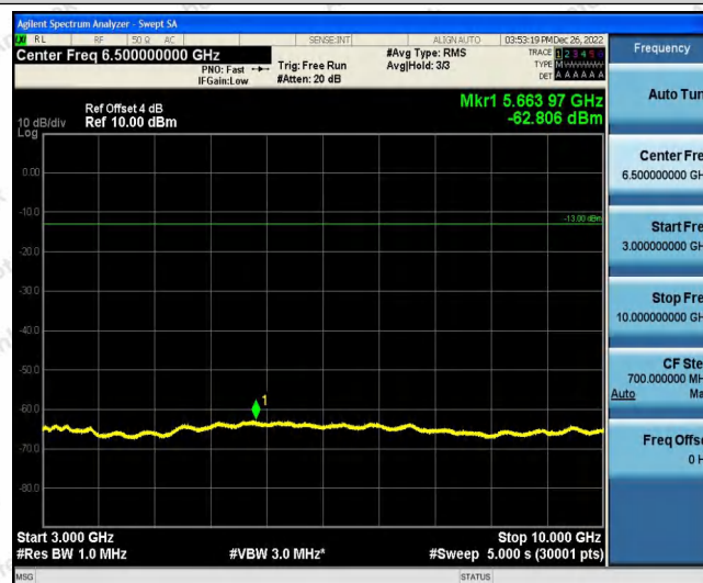
Band5-4182-10000~18000MHz
