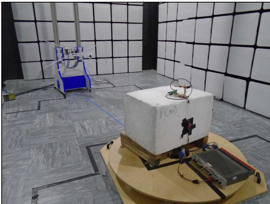
Figure 1 - 30 MHz to 1 GHz, Coil Antenna
