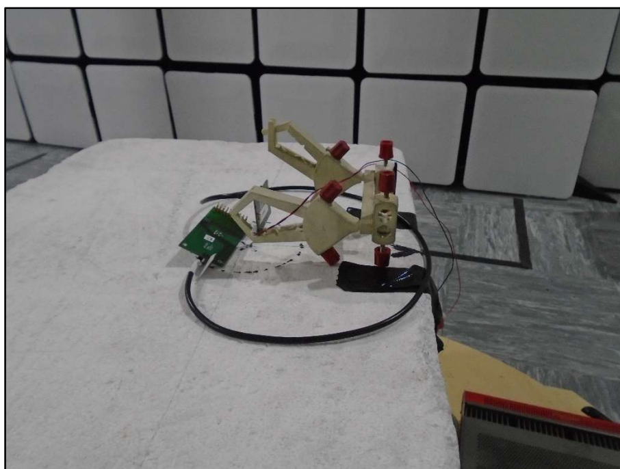
Figure 4 - Coil Antenna, Orientation Y
