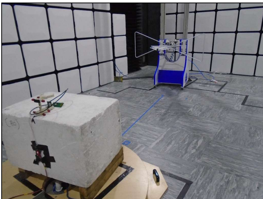
Figure 5 - Coil Antenna, Orientation Z
