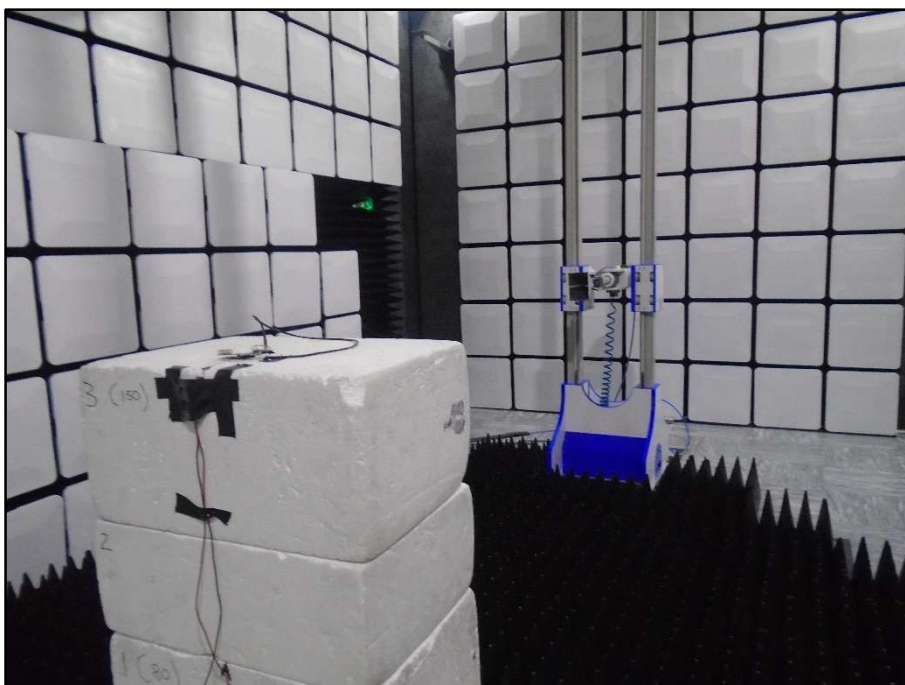
Figure 2 - 1 GHz to 5 GHz, Coil Antenna
