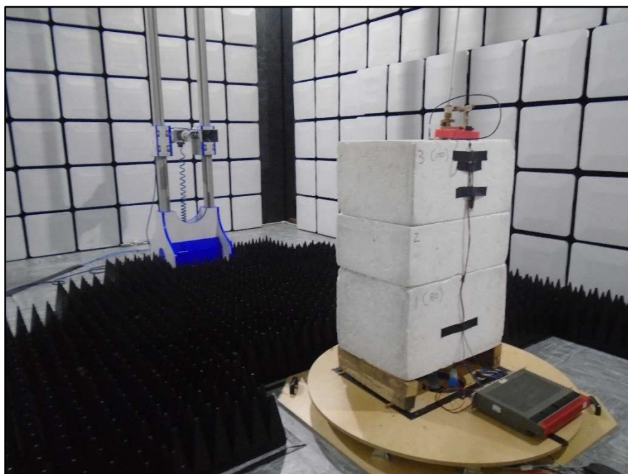
Figure 7 - 1 GHz to 5 GHz, Dipole Stick Antenna
