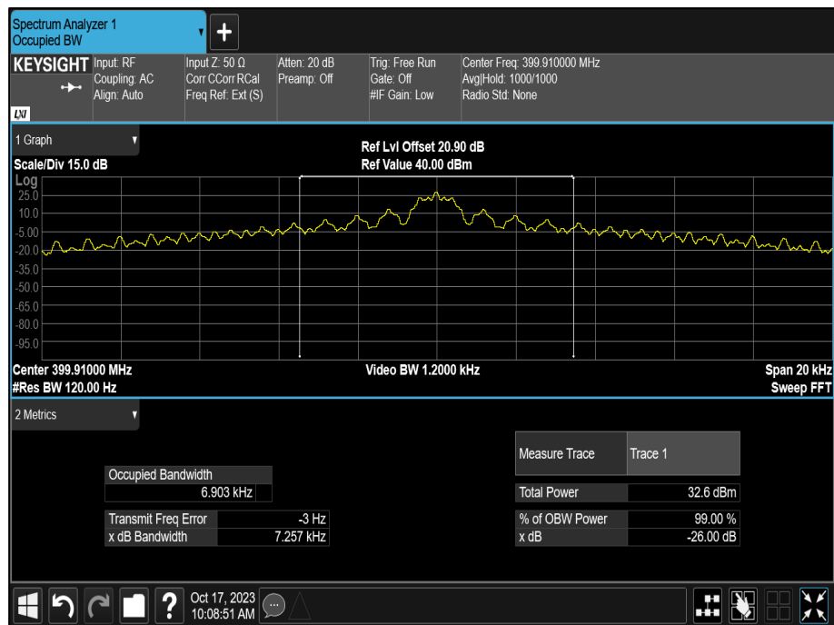
Figure 26 - 399.91 MHz
