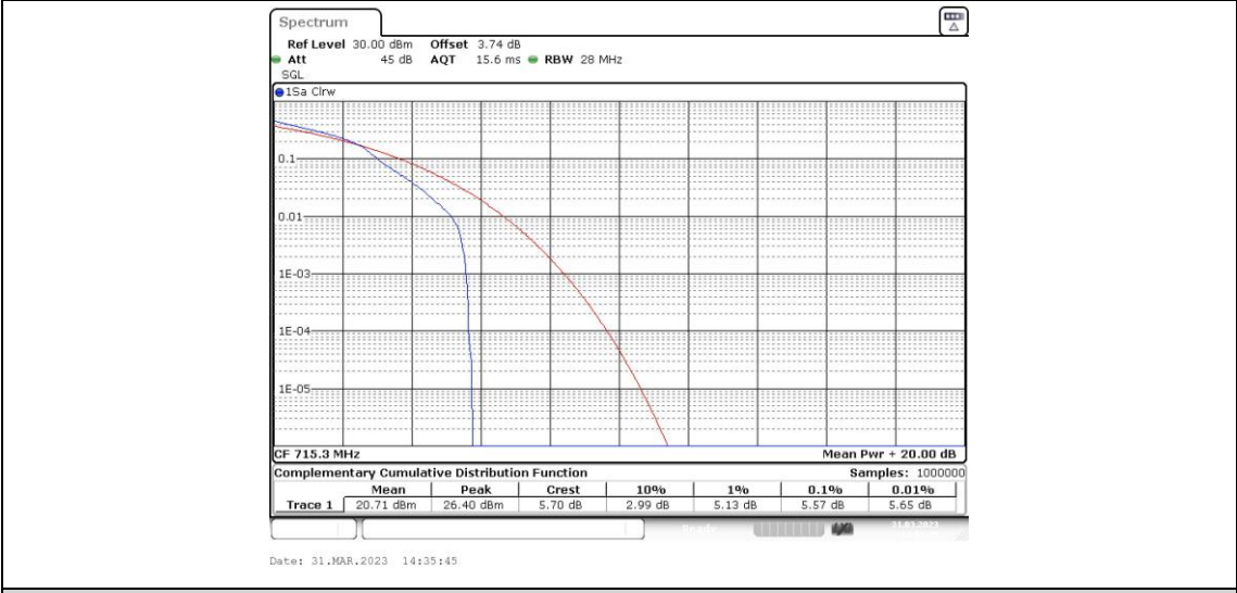
Band12-1.4MHz-16QAM-23173-6RB#0
