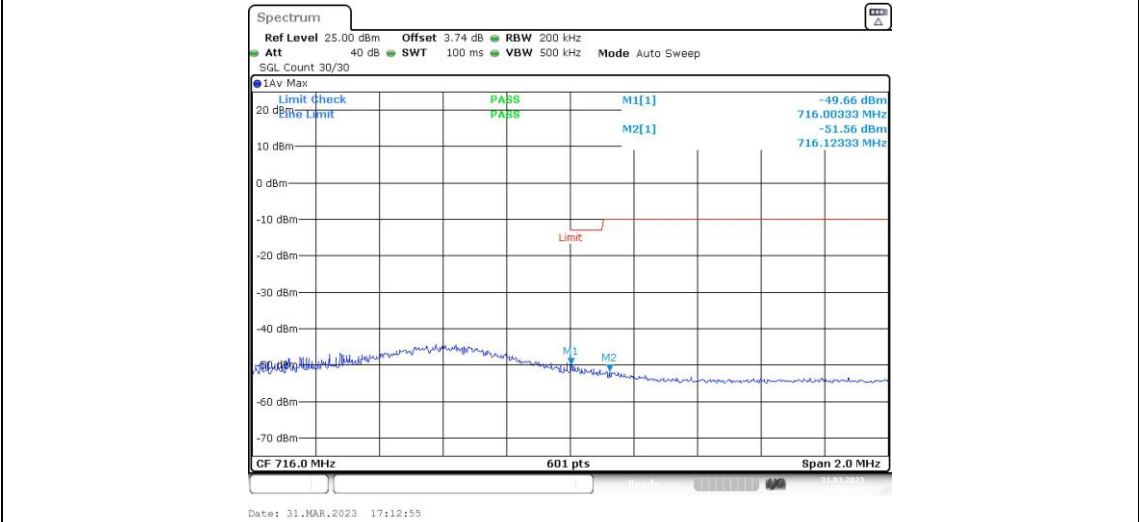
Band12-10MHz-QPSK-23130-1RB#49
