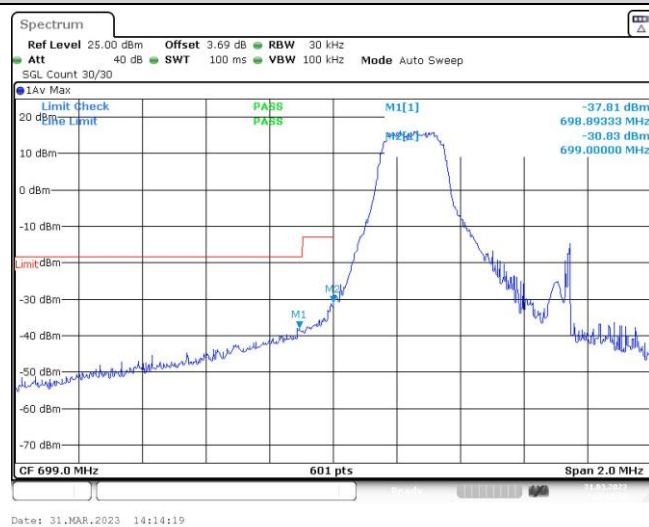
Band12-1.4MHz-16QAM-23017-1RB#5
