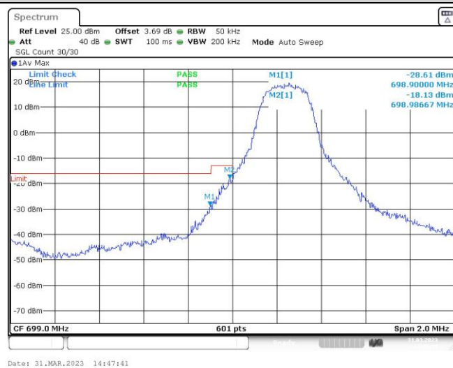
Band12-3MHz-QPSK-23025-1RB#14
