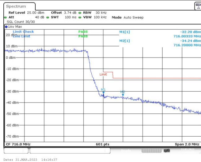
Band12-3MHz-QPSK-23025-1RB#0
