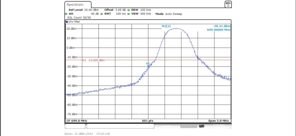
Band12-5MHz-QPSK-23035-1RB#24
