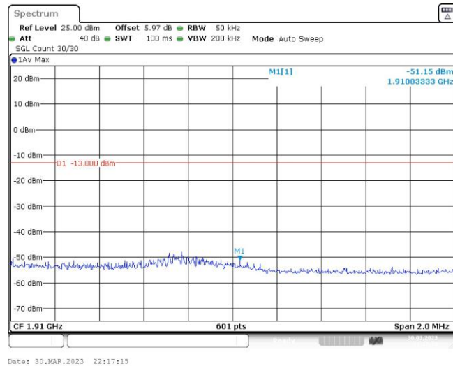
Band2-3MHz-16QAM-19185-1RB#14
