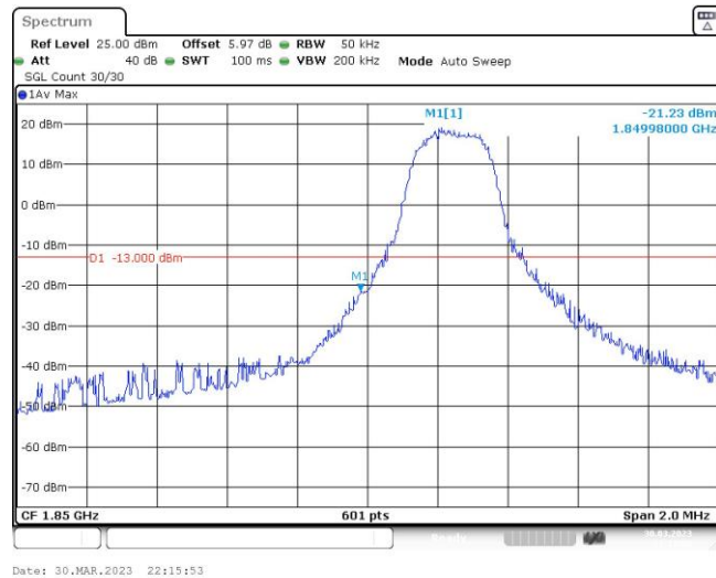
Band2-3MHz-16QAM-18615-1RB#14
