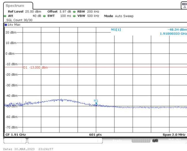
Band2-10MHz-QPSK-19150-1RB#49
