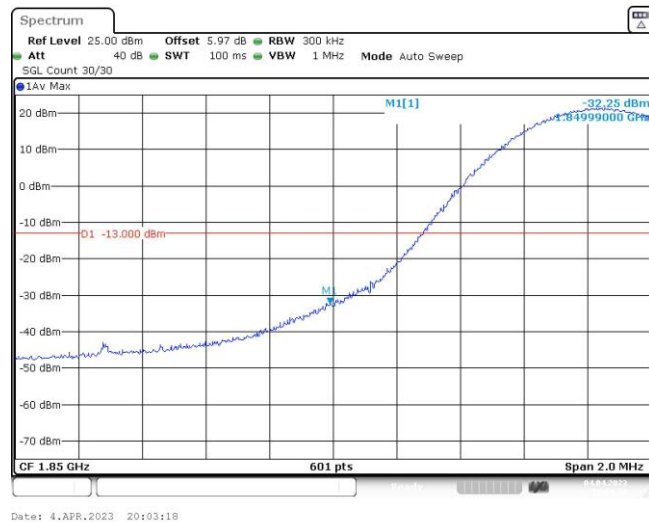
Band25-15MHz-16QAM-26115-1RB#74
