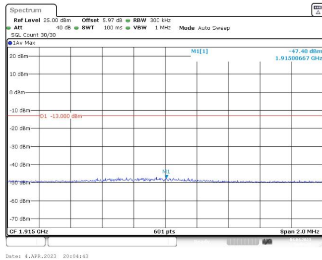
Band25-15MHz-16QAM-26615-1RB#74
