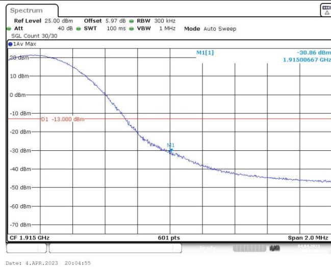
Band25-15MHz-QPSK-26615-75RB#0
