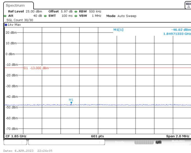
Band25-20MHz-16QAM-26140-100RB#0
