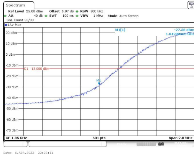
Band25-20MHz-16QAM-26140-1RB#99
