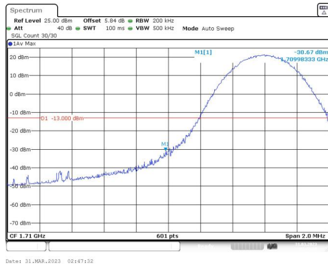
Band4-10MHz-16QAM-20000-1RB#49
