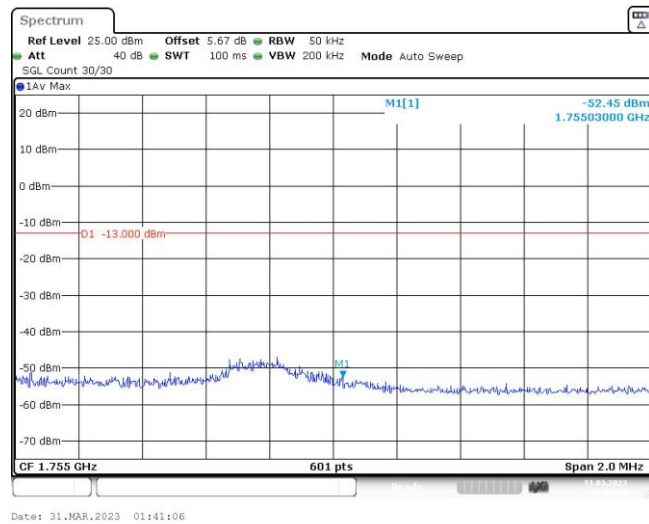
Band4-3MHz-16QAM-20385-1RB#14
