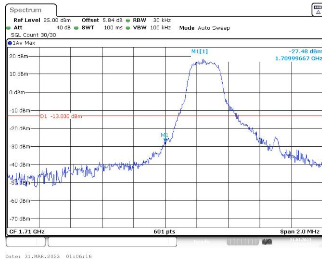
Band4-1.4MHz-QPSK-19957-1RB#5
