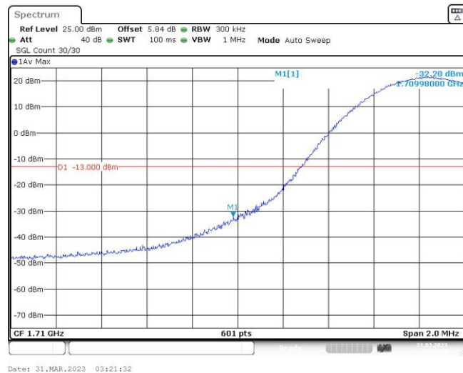
Band4-15MHz-16QAM-20025-1RB#74
