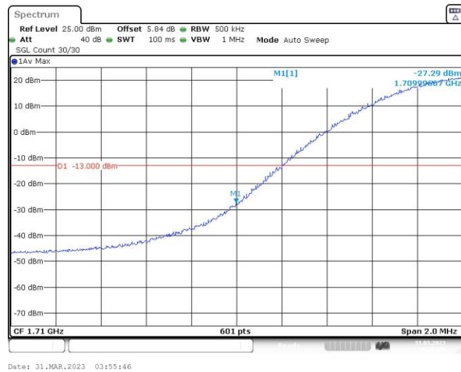
Band4-20MHz-16QAM-20050-1RB#99
