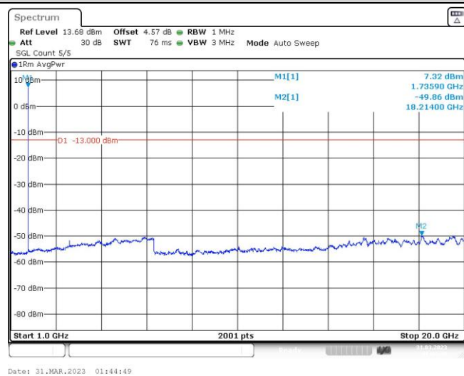
Band4-3MHz-QPSK-20385-1RB#0-Range1:0.009~0.15MHz
