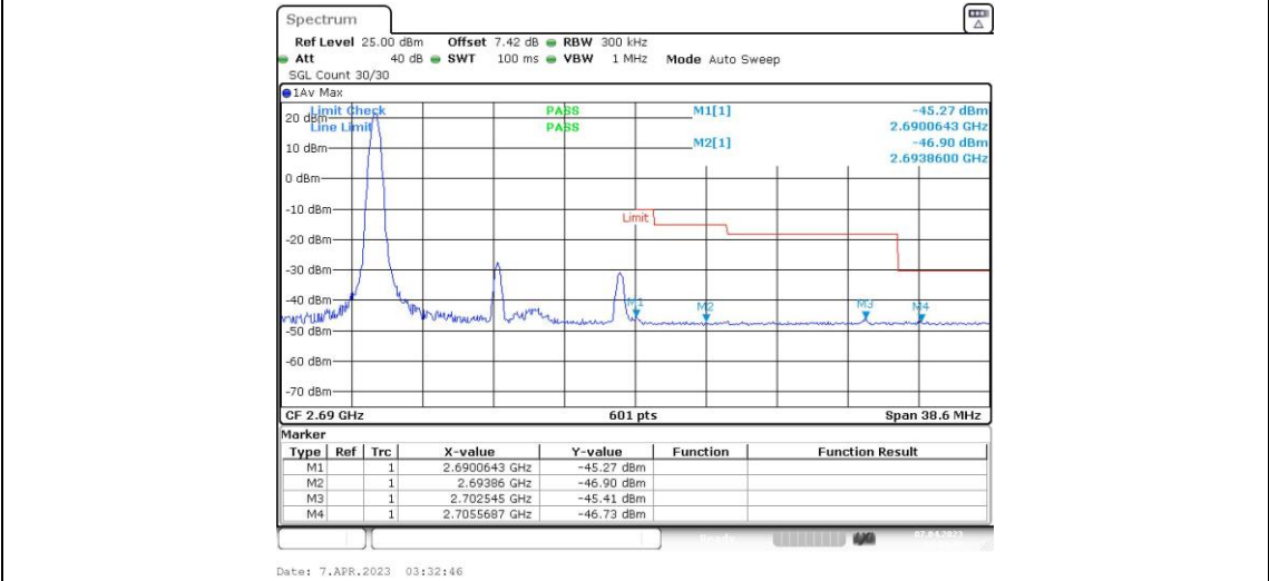
Band41-15MHz-QPSK-41515-1RB#74
