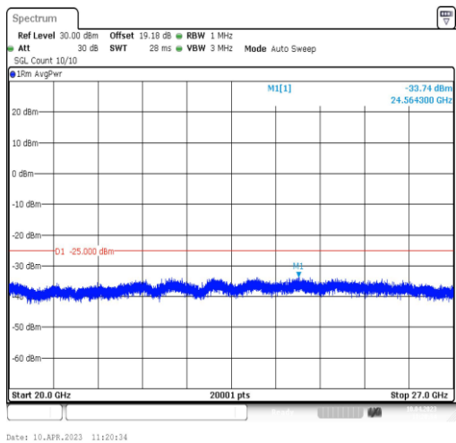
15MHz-15MHz-37925-38075
