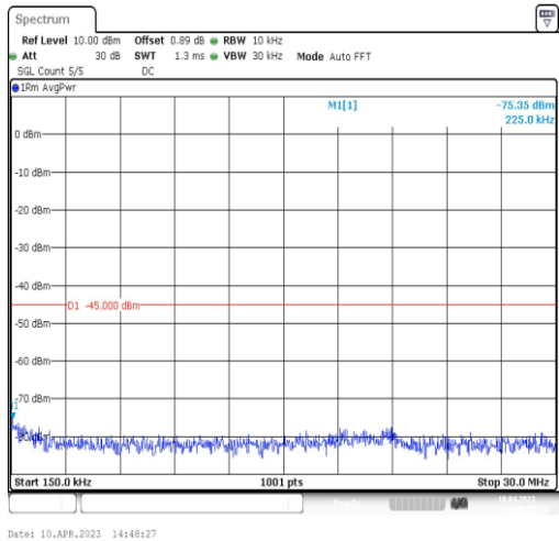
41-41-5MHz-20MHz-QPSK-QPSK-39683-39800-1RB#0-0RB#0-0.15~30MHz
