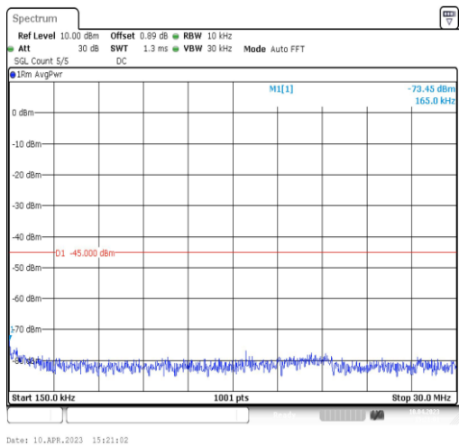
41-41-5MHz-20MHz-QPSK-QPSK-41373-41490-1RB#0-0RB#0-0.15~30MHz
