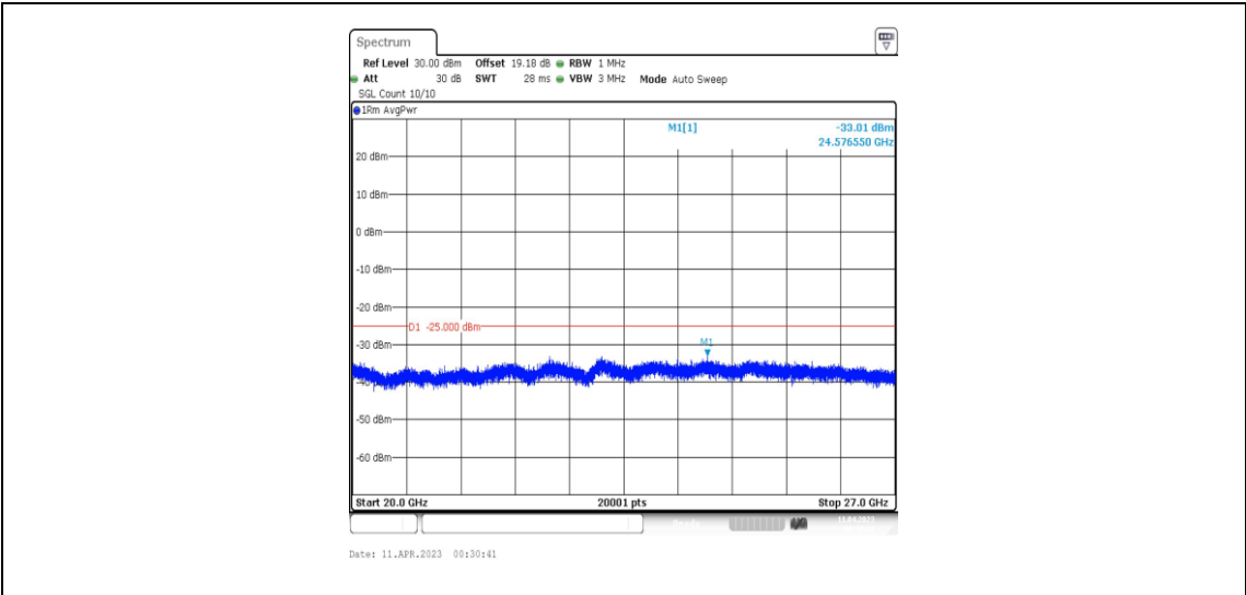
41-41-15MHz-15MHz-QPSK-QPSK-39725-39875-75RB#0-75RB#0-20000~27000MHz
