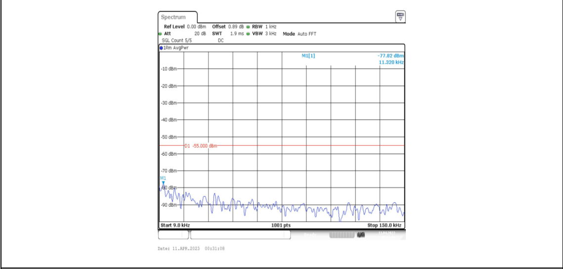
41-41-15MHz-15MHz-16QAM-16QAM-39725-39875-75RB#0-75RB#0-0.009~0.15MHz
