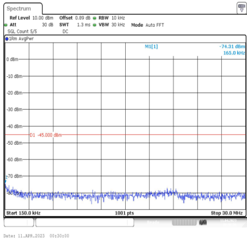
41-41-15MHz-15MHz-QPSK-QPSK-39725-39875-75RB#0-75RB#0-0.15~30MHz
