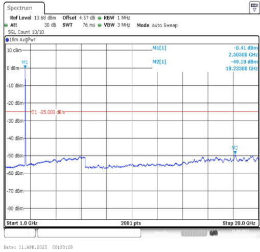
41-41-15MHz-15MHz-QPSK-QPSK-39725-39875-75RB#0-75RB#0-1000~20000MHz
