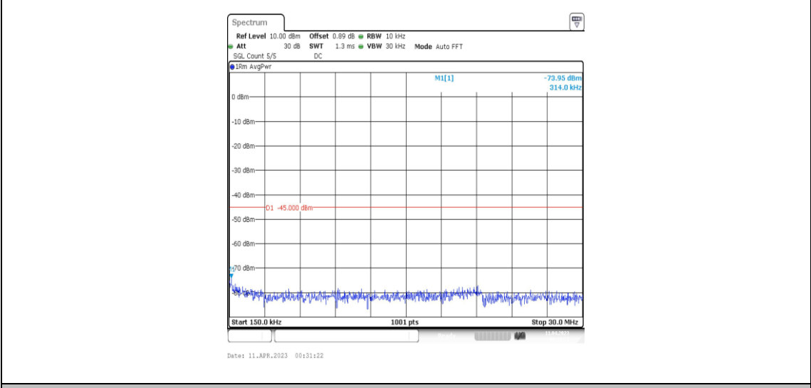
41-41-15MHz-15MHz-16QAM-16QAM-39725-39875-75RB#0-75RB#0-0.15~30MHz
