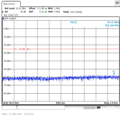
41-41-15MHz-15MHz-QPSK-QPSK-39725-39875-75RB#0-75RB#0-30~1000MHz
