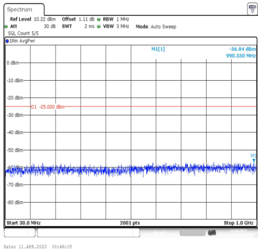
41-41-15MHz-15MHz-QPSK-QPSK-40545-40695-75RB#0-75RB#0-30~1000MHz
