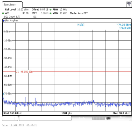
41-41-15MHz-15MHz-QPSK-QPSK-40545-40695-75RB#0-75RB#0-0.15~30MHz
