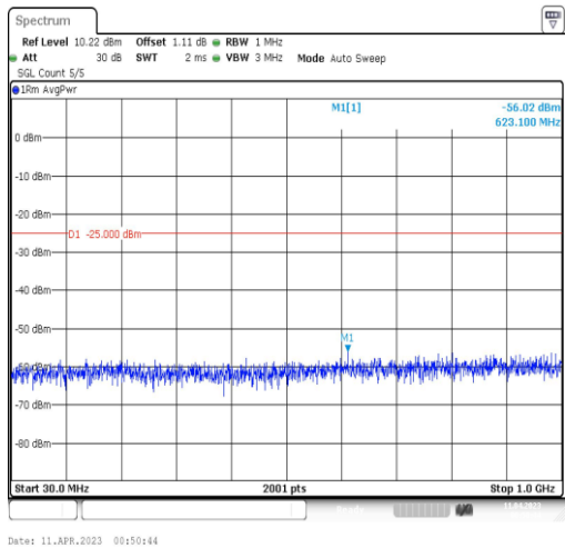
41-41-15MHz-15MHz-QPSK-QPSK-41365-41515-1RB#0-0RB#0-30~1000MHz
