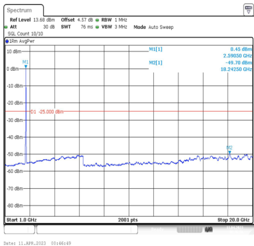
41-41-15MHz-15MHz-QPSK-QPSK-40545-40695-75RB#0-75RB#0-1000~20000MHz
