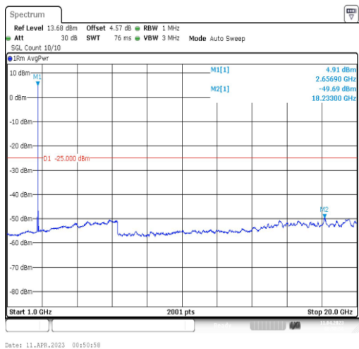
41-41-15MHz-15MHz-QPSK-QPSK-41365-41515-1RB#0-0RB#0-1000~20000MHz
