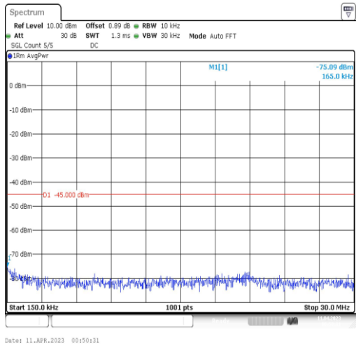
41-41-15MHz-15MHz-QPSK-QPSK-41365-41515-1RB#0-0RB#0-0.15~30MHz
