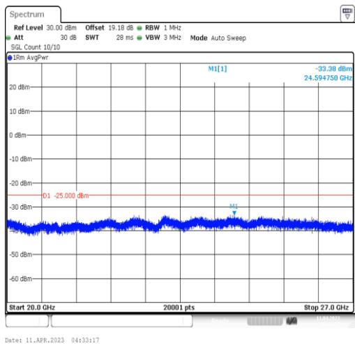
41-41-20MHz-5MHz-16QAM-16QAM-40595-40712-1RB#0-0RB#0-20000~27000MHz
