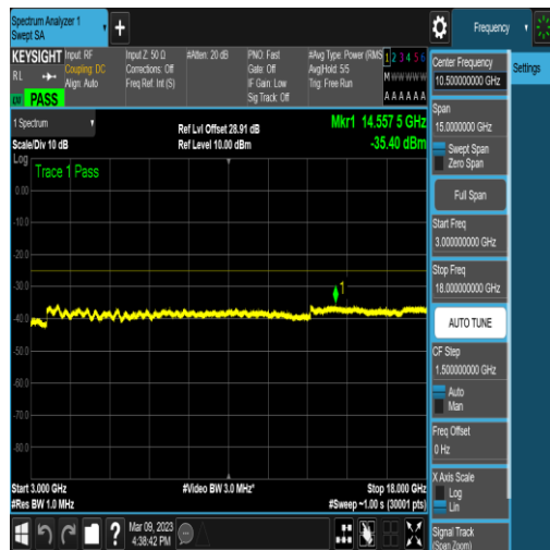
NTNV_N41_PC2_30_20_H_TID18_N/A_3000_18 000_#1
