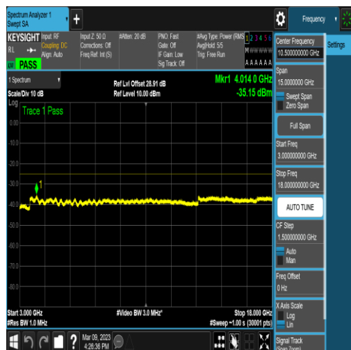
NTNV_N41_PC2_30_20_M_TID17_N/A_3000_18 000_#1
