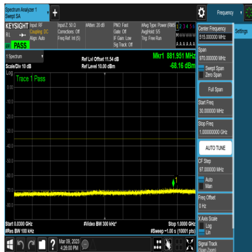
NTNV_N41_PC2_30_20_M_TID17_N/A_30_1000 _#1
