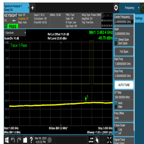
NTNV_N41_PC2_30_20_M_TID6_N/A_1000_300_0_#1
