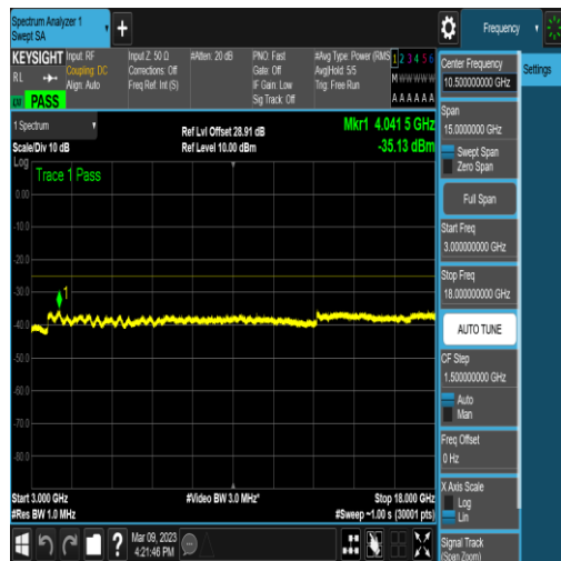
NTNV_N41_PC2_30_20_M_TID5_N/A_3000_18000_#1
