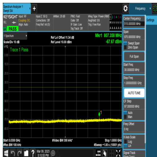
NTNV_N41_PC2_30_40_H_TID16_N/A_30_1000_#1
