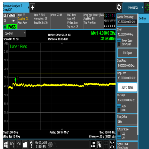
NTNV_N41_PC2_30_60_L_TID5_N/A_3000_18000_#1
