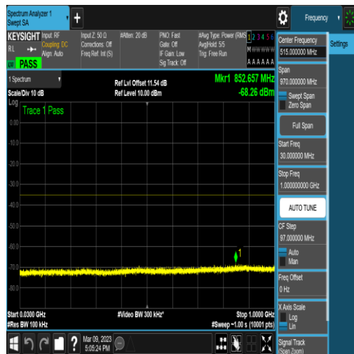
NTNV_N41_PC2_30_40_H_TID4_N/A_30_1000_ #1
