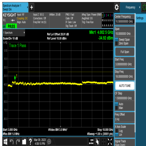
NTNV_N41_PC2_30_40_M_TID16_N/A_3000_18 000_#1
