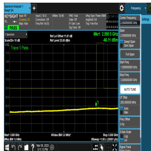
NTNV_N41_PC2_30_40_H_TID16_N/A_1000_3000_#1
