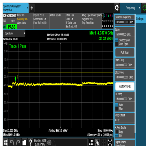
NTNV_N41_PC2_30_40_H_TID18_N/A_3000_18 000_#1
