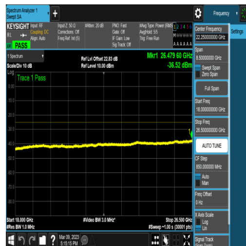
NTNV_N41_PC2_30_40_H_TID18_N/A_18000_2 6500_#1
