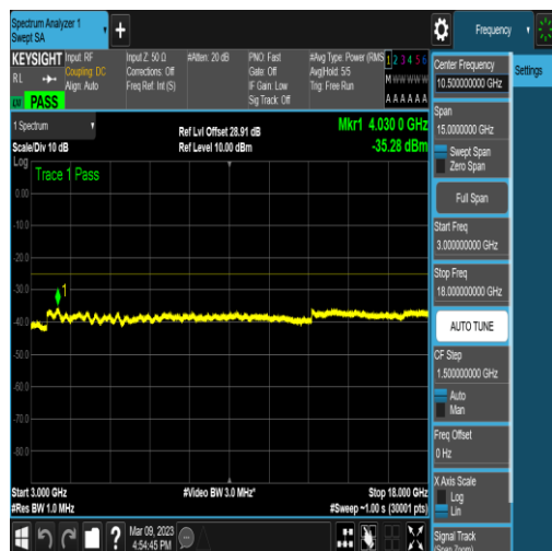
NTNV_N41_PC2_30_40_M_TID5_N/A_3000_180 00_#1
