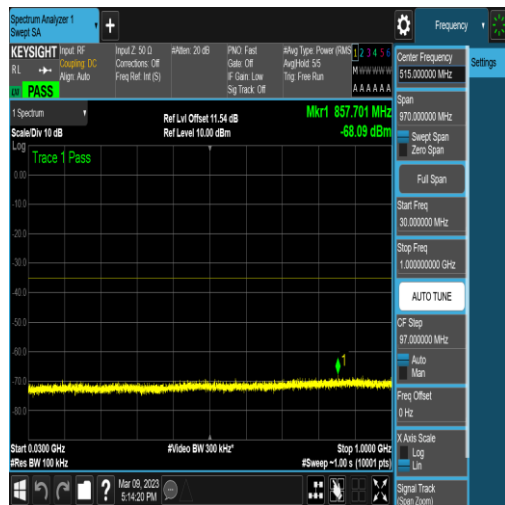
NTNV_N41_PC2_30_40_H_TID18_N/A_30_1000 _#1
