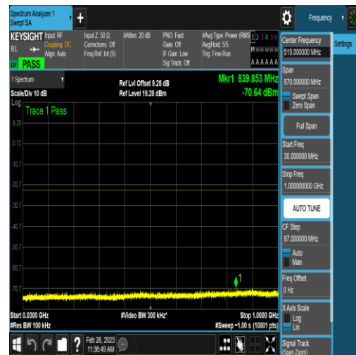
NTNV_N77-3700-3980_PC2_30_100_H_TID18_N S_01_30_1000_#1
