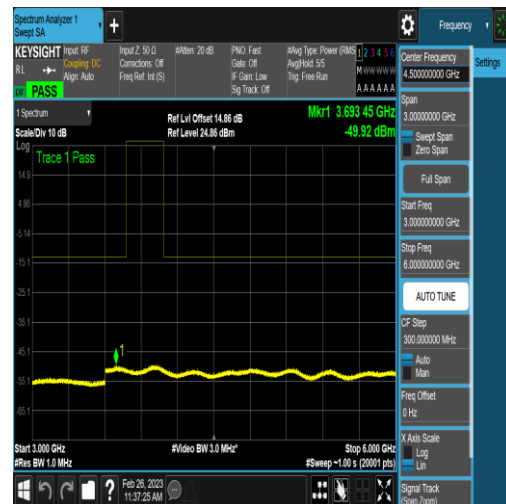
NTNV_N77-3700-3980_PC2_30_100_H_TID18_N S_01_3000_6000_#1
