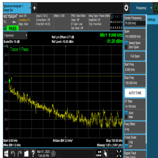
NTNV_N78-3450-3550_PC2_30_60_H_TID5_N/A _0.009_0.15_#1
