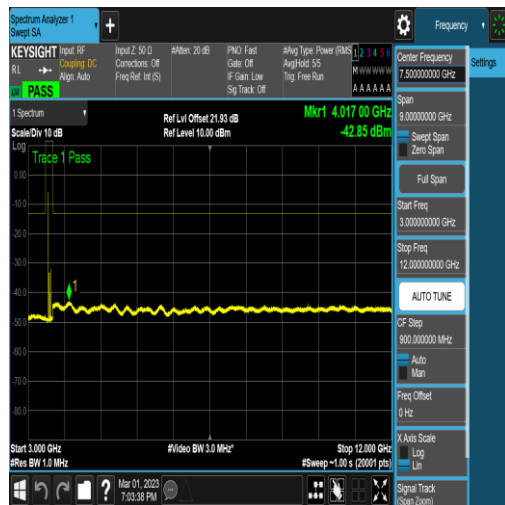
NTNV_N78-3450-3550_PC2_30_60_H_TID4_N/A _3000_12000_#1
