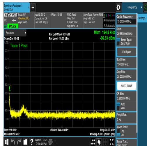
NTNV_N78-3450-3550_PC2_30_60_H_TID5_N/A _0.15_30_#1
