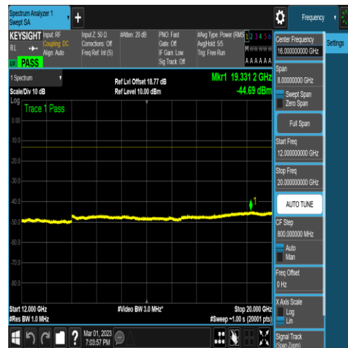
NTNV_N78-3450-3550_PC2_30_60_H_TID4_N/A _12000_20000_#1
