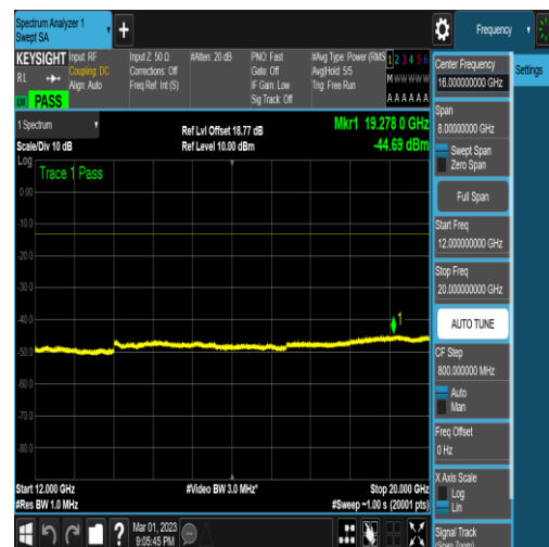
NTNV_N78-3450-3550_PC2_30_100_H_TID16_N /A_12000_20000_#1
