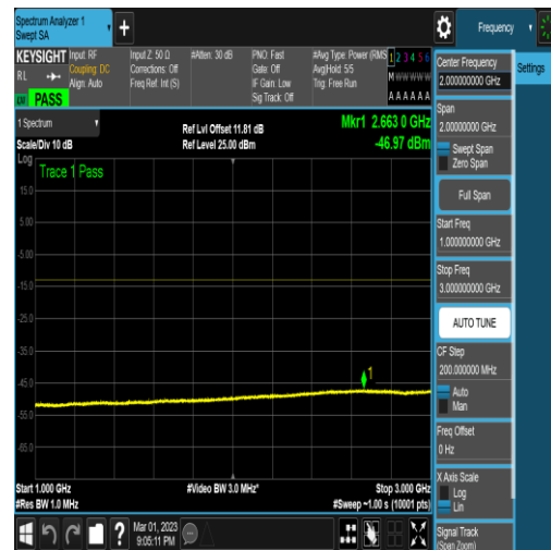
NTNV_N78-3450-3550_PC2_30_100_H_TID16_N /A_1000_3000_#1
