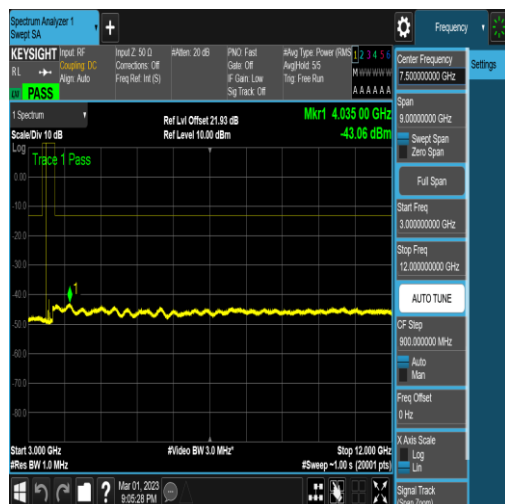
NTNV_N78-3450-3550_PC2_30_100_H_TID16_N /A_3000_12000_#1
