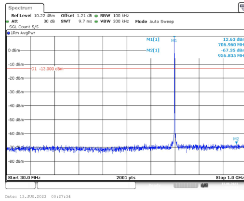
Band12-1.4MHz-QPSK-23095-1RB#0-Range3:30~1000MHz
