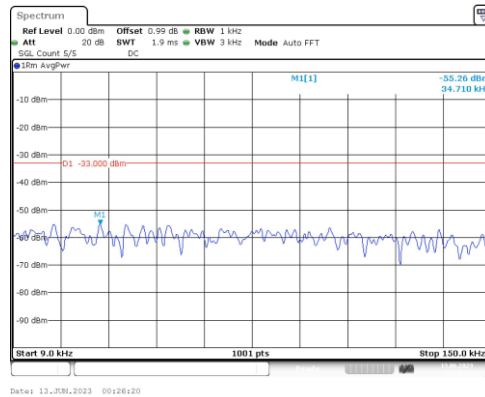
Band12-1.4MHz-16QAM-23017-1RB#0-Range1:0.009~0.15MHz
