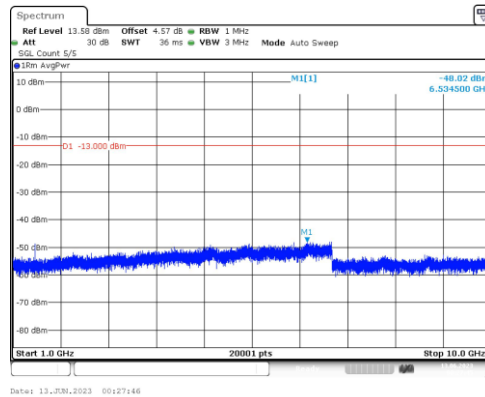
Band12-1.4MHz-QPSK-23095-1RB#0-Range4:1000~10000MHz
