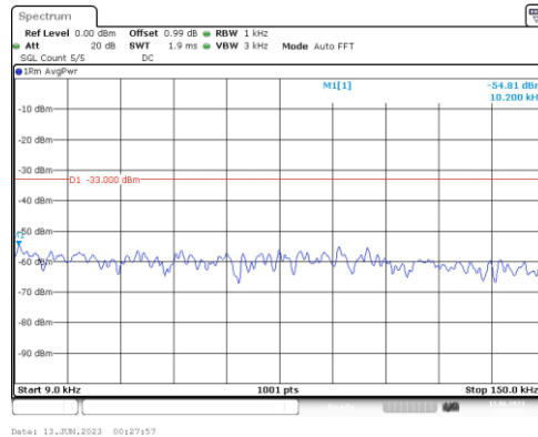
Band12-1.4MHz-16QAM-23095-1RB#0-Range1:0.009~0.15MHz
