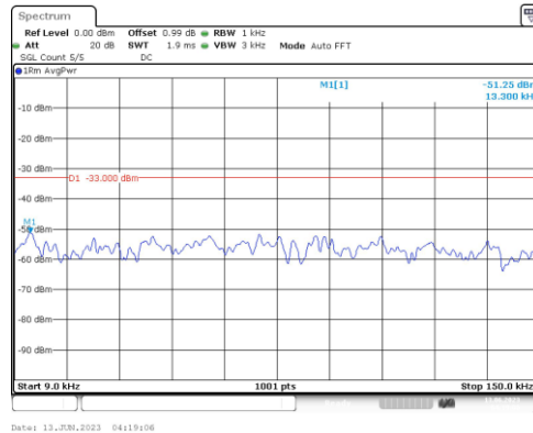
Band17-10MHz-QPSK-23800-1RB#0-Range1:0.009~0.15MHz
