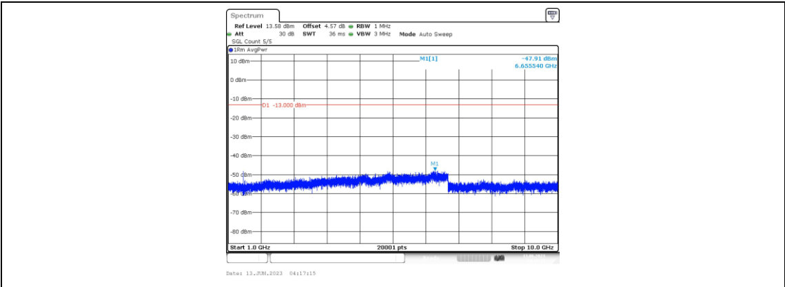
Band17-10MHz-16QAM-23780-1RB#0-Range4:1000~10000MHz
