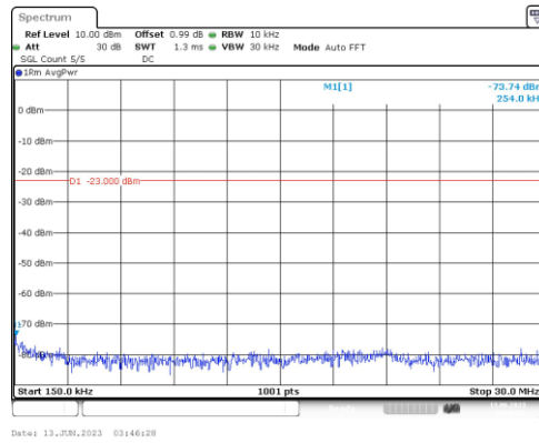
Band17-5MHz-QPSK-23825-1RB#0-Range2:0.15~30MHz
