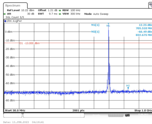
Band17-10MHz-16QAM-23790-1RB#0-Range3:30~1000MHz
