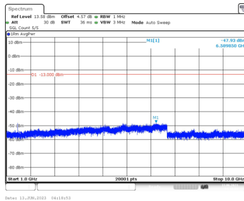
Band17-10MHz-16QAM-23790-1RB#0-Range4:1000~10000MHz
