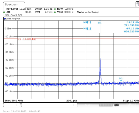
Band17-5MHz-QPSK-23825-1RB#0-Range3:30~1000MHz
