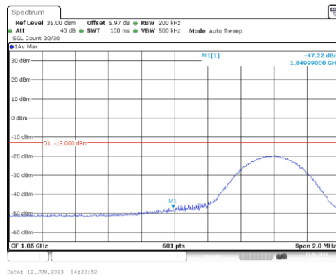
Band2-10MHz-16QAM-18650-1RB#49
