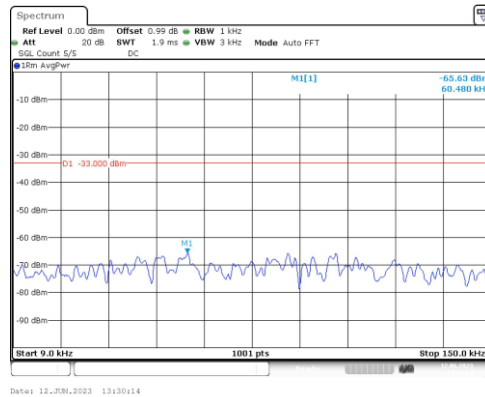
Band2-3MHz-QPSK-18900-1RB#0-Range1:0.009~0.15MHz
