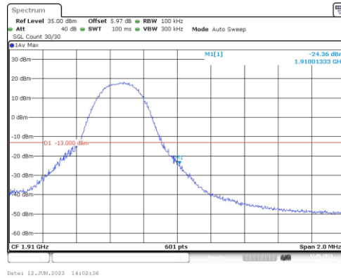
Band2-5MHz-16QAM-19175-1RB#24
