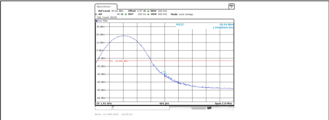
Band2-10MHz-16QAM-19150-1RB#49
