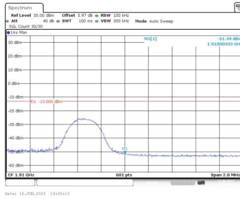
Band2-5MHz-16QAM-19175-1RB#0
