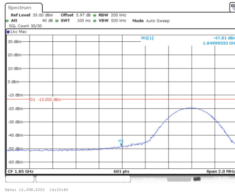
Band2-10MHz-QPSK-18650-1RB#49
