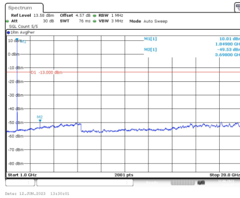
Band2-3MHz-16QAM-18615-1RB#0-Range4:1000~20000MHz
