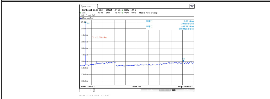
Band2-3MHz-16QAM-18900-1RB#0-Range4:1000~20000MHz
