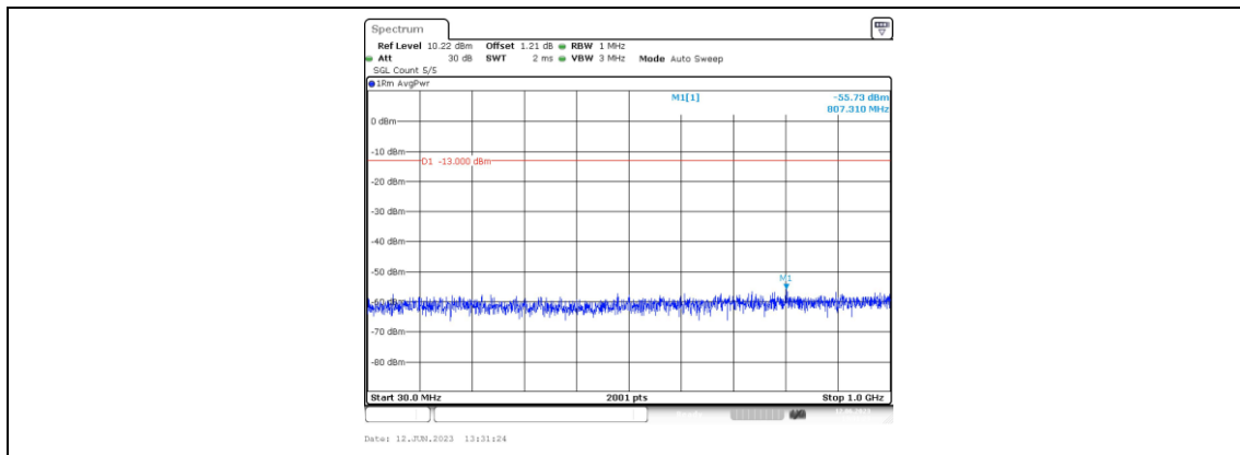
Band2-3MHz-16QAM-18900-1RB#0-Range3:30~1000MHz
