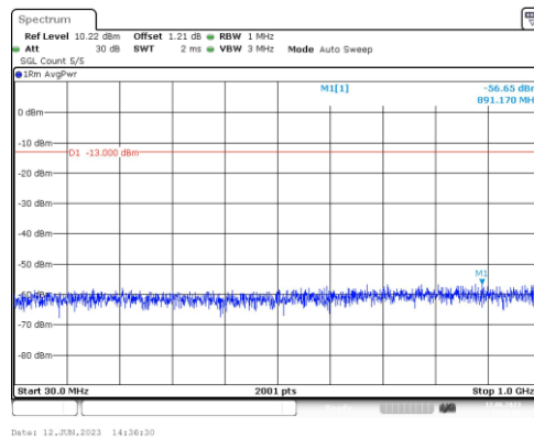
Band2-10MHz-QPSK-18650-1RB#0-Range3:30~1000MHz
