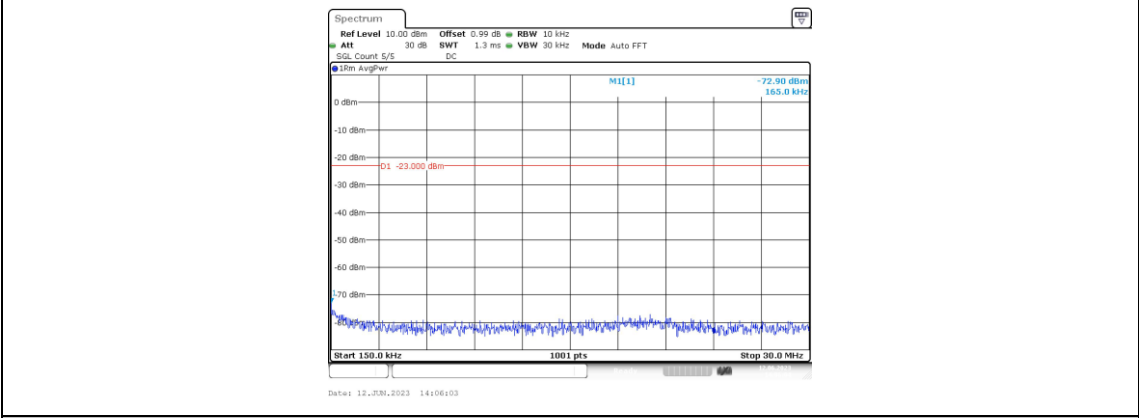
Band2-5MHz-16QAM-18900-1RB#0-Range2:0.15~30MHz
