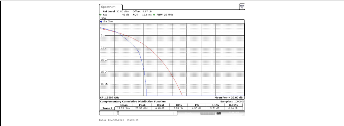
Band25-1.4MHz-16QAM-26047-6RB#0
