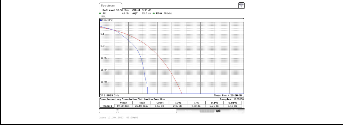
Band25-3MHz-16QAM-26365-15RB#0
