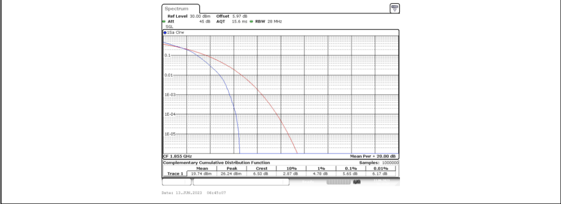
Band25-10MHz-16QAM-26090-50RB#0
