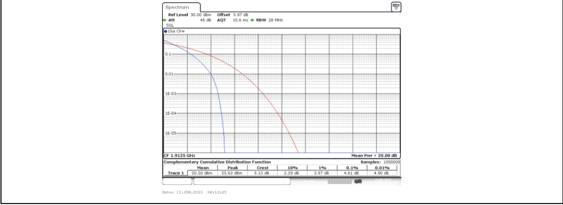
Band25-5MHz-16QAM-26665-1RB#0
