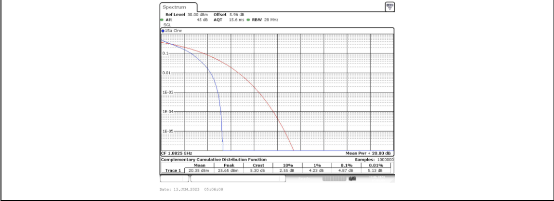
Band25-1.4MHz-16QAM-26365-1RB#0
