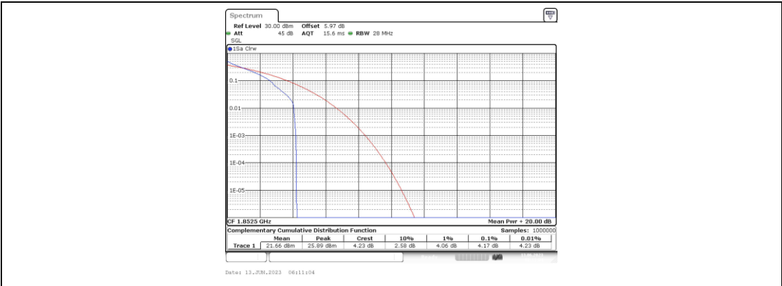
Band25-5MHz-QPSK-26065-1RB#0
