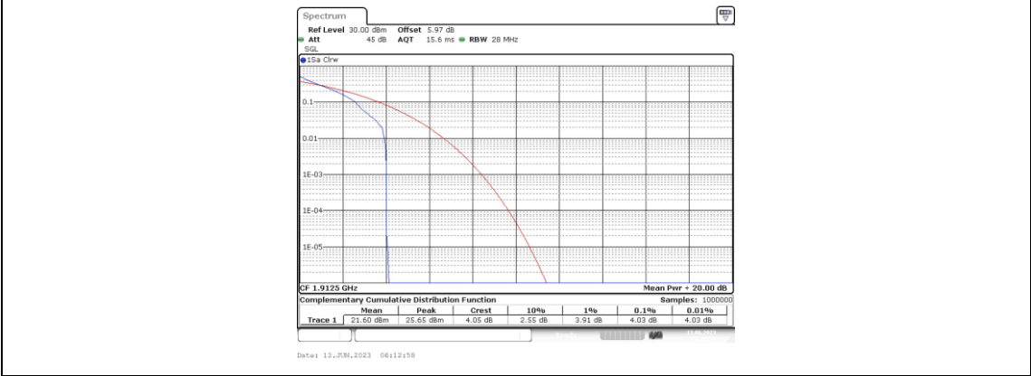
Band25-5MHz-QPSK-26665-1RB#0
