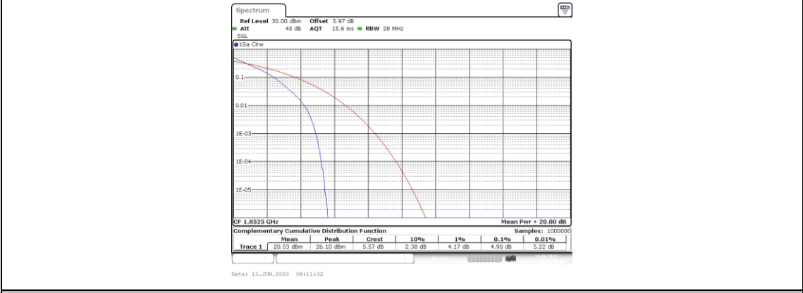
Band25-5MHz-QPSK-26065-25RB#0
