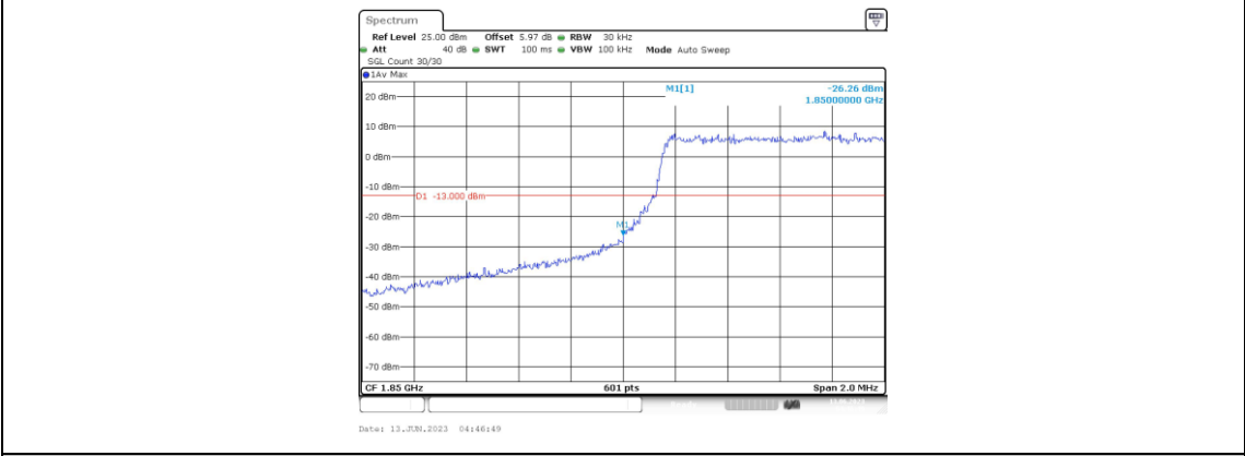
Band25-1.4MHz-16QAM-26047-6RB#0
